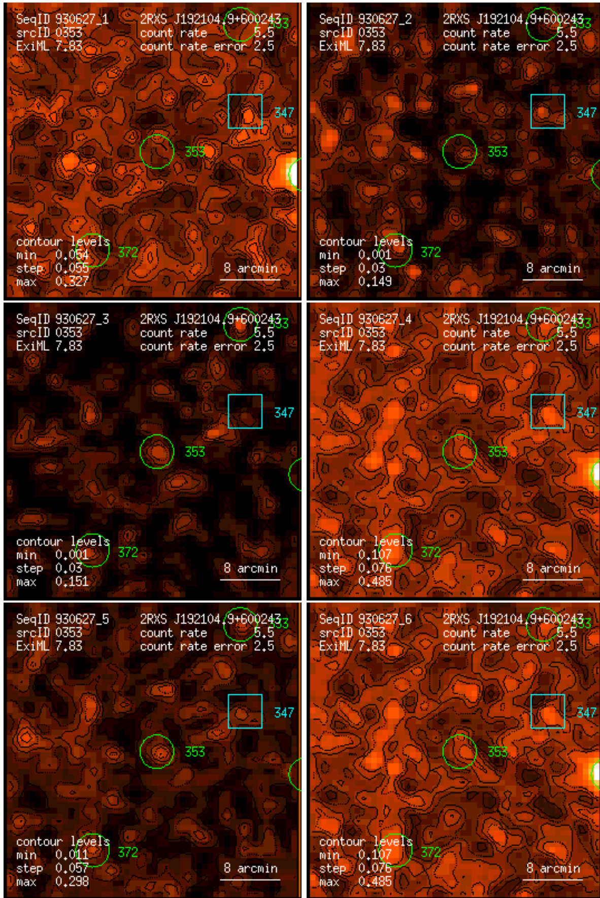
Figure 353: RASS 930627: detection 0353: band rate images, Gaussian filter: (1) PSPC channels 11 – 41, (2) 52 – 90, (3) 91 – 201, (4) 11 – 235, (5) 52 – 201, (6) 11 – 201. Broad band rates in counts/ks. Band rate contour levels in counts/ks/arcmin 2 .
