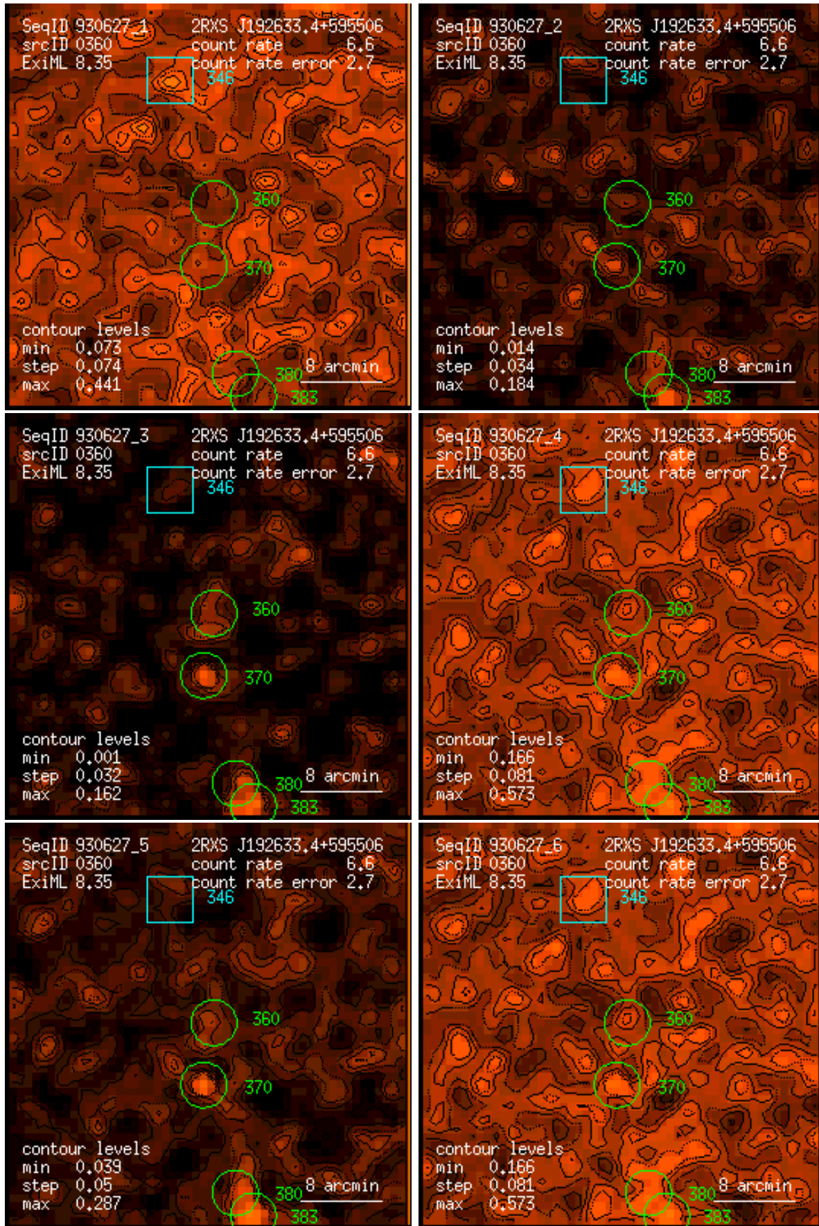
Figure 360: RASS 930627: detection 0360: band rate images, Gaussian filter: (1) PSPC channels 11 – 41, (2) 52 – 90, (3) 91 – 201, (4) 11 – 235, (5) 52 – 201, (6) 11 – 201. Broad band rates in counts/ks. Band rate contour levels in counts/ks/arcmin 2 .
