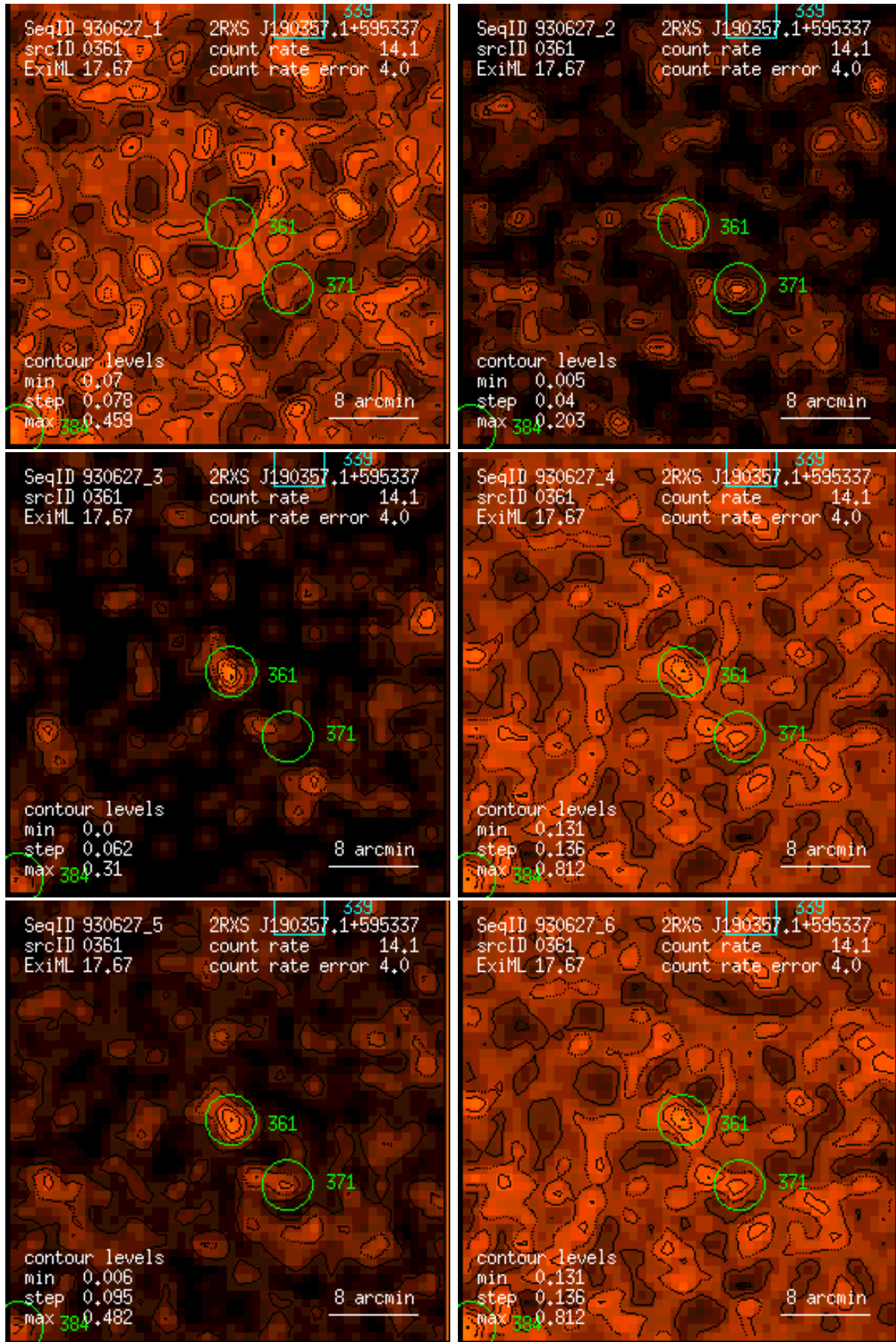
Figure 361: RASS 930627: detection 0361: band rate images, Gaussian filter: (1) PSPC channels 11 – 41, (2) 52 – 90, (3) 91 – 201, (4) 11 – 235, (5) 52 – 201, (6) 11 – 201. Broad band rates in counts/ks. Band rate contour levels in counts/ks/arcmin 2 .
