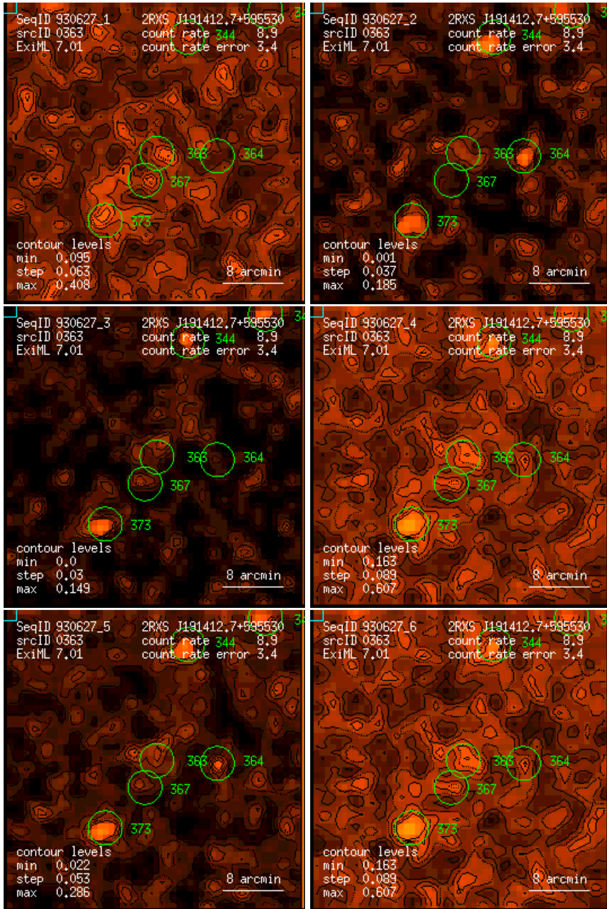
Figure 363: RASS 930627: detection 0363: band rate images, Gaussian filter: (1) PSPC channels 11 – 41, (2) 52 – 90, (3) 91 – 201, (4) 11 – 235, (5) 52 – 201, (6) 11 – 201. Broad band rates in counts/ks. Band rate contour levels in counts/ks/arcmin 2 .
