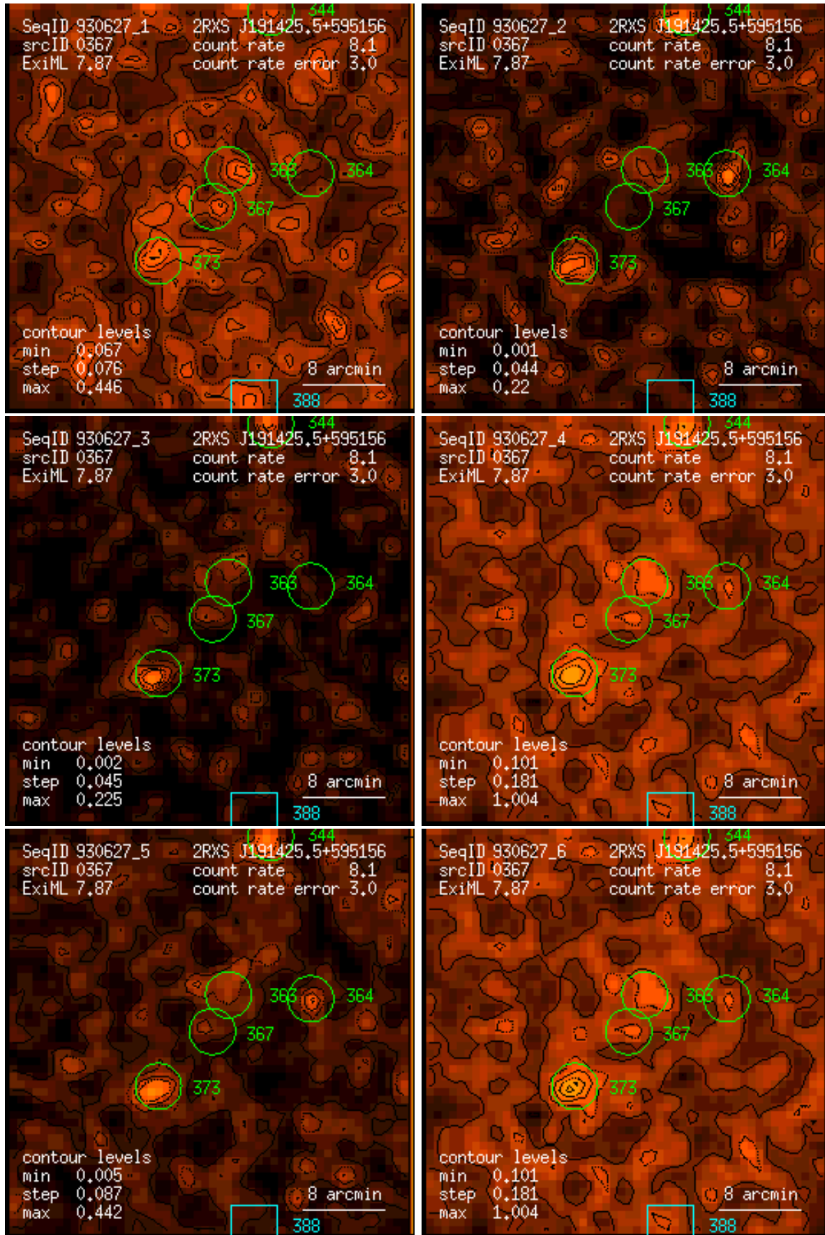
Figure 367: RASS 930627: detection 0367: band rate images, Gaussian filter: (1) PSPC channels 11 – 41, (2) 52 – 90, (3) 91 – 201, (4) 11 – 235, (5) 52 – 201, (6) 11 – 201. Broad band rates in counts/ks. Band rate contour levels in counts/ks/arcmin 2 .
