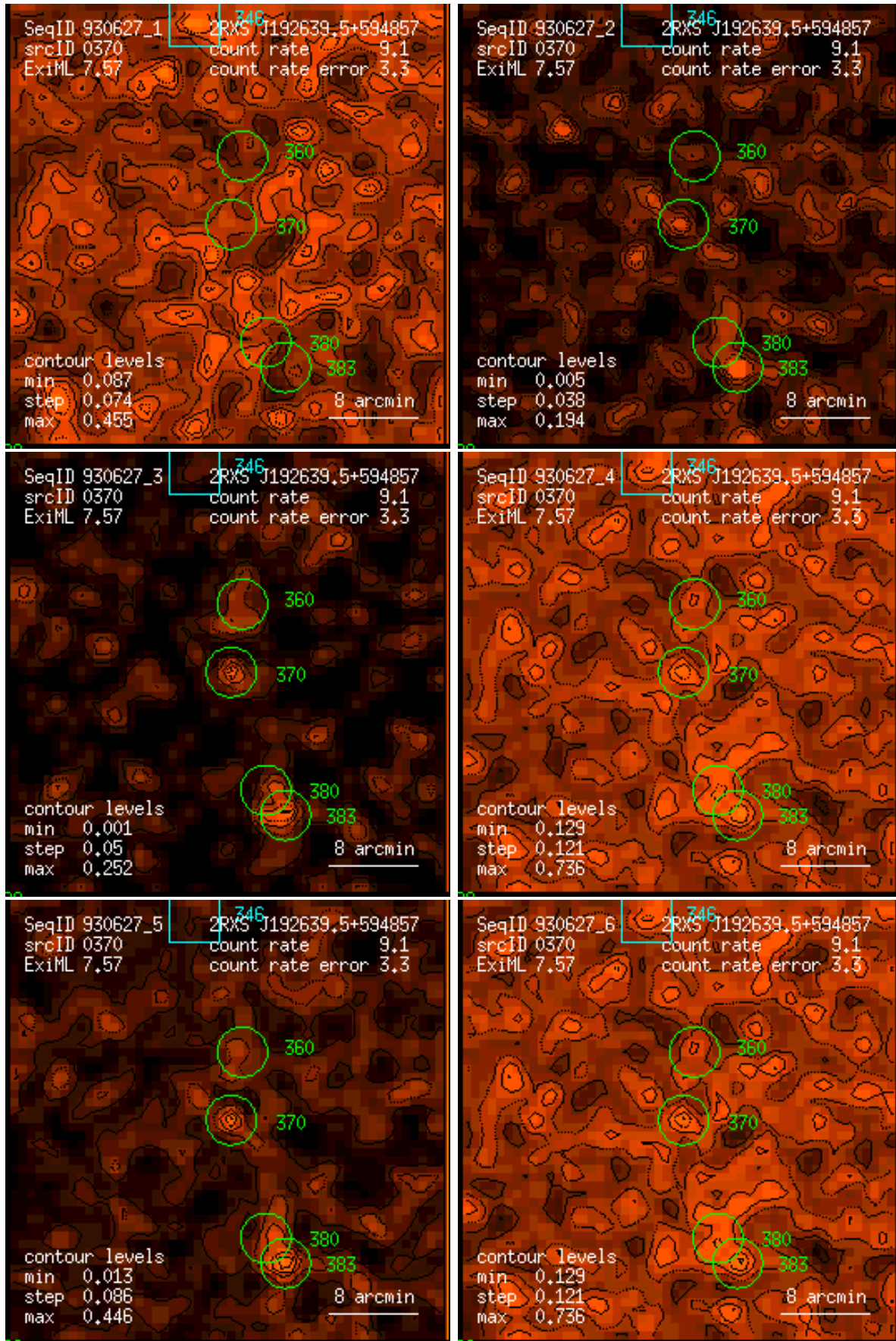
Figure 370: RASS 930627: detection 0370: band rate images, Gaussian filter: (1) PSPC channels 11 – 41, (2) 52 – 90, (3) 91 – 201, (4) 11 – 235, (5) 52 – 201, (6) 11 – 201. Broad band rates in counts/ks. Band rate contour levels in counts/ks/arcmin 2 .
