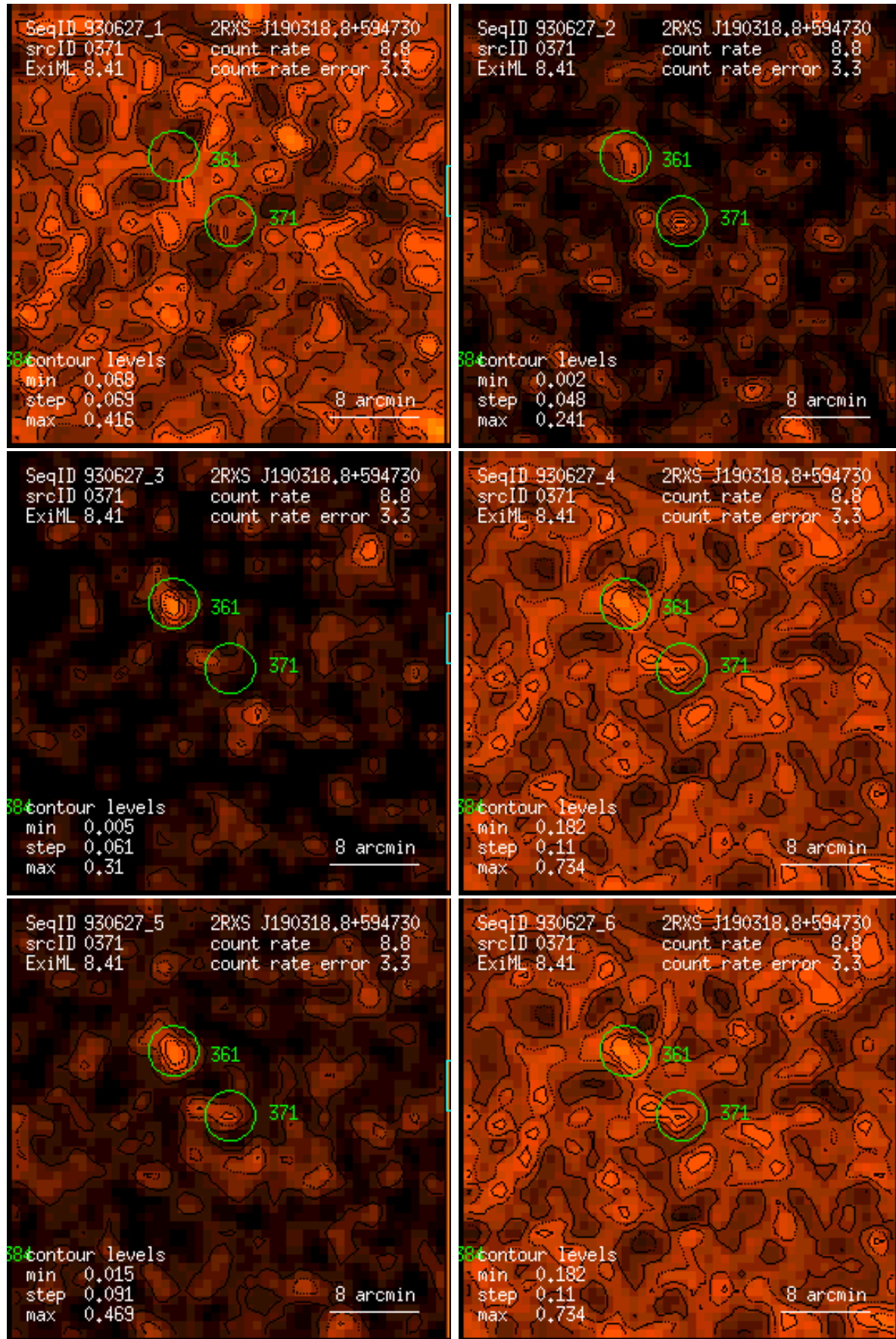
Figure 371: RASS 930627: detection 0371: band rate images, Gaussian filter: (1) PSPC channels 11 – 41, (2) 52 – 90, (3) 91 – 201, (4) 11 – 235, (5) 52 – 201, (6) 11 – 201. Broad band rates in counts/ks. Band rate contour levels in counts/ks/arcmin 2 .
