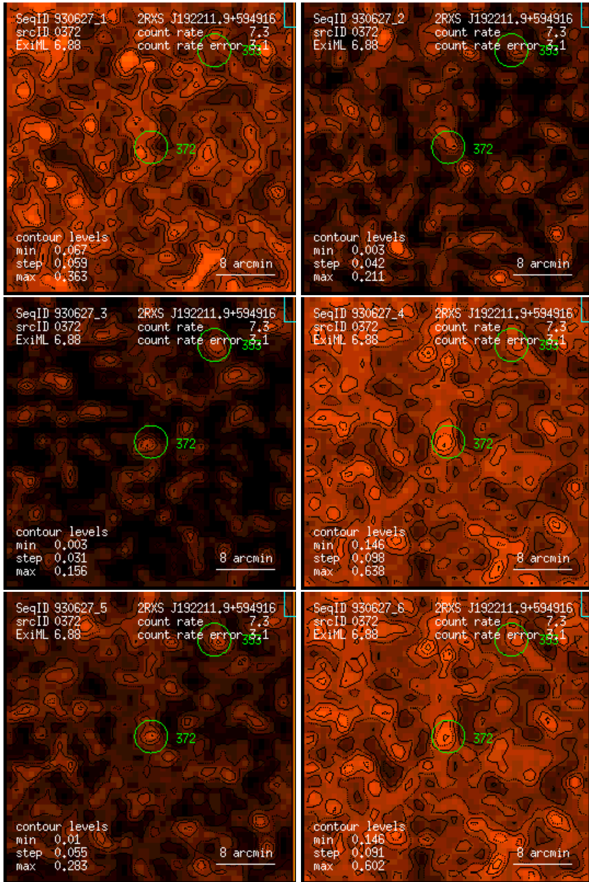
Figure 372: RASS 930627: detection 0372: band rate images, Gaussian filter: (1) PSPC channels 11 – 41, (2) 52 – 90, (3) 91 – 201, (4) 11 – 235, (5) 52 – 201, (6) 11 – 201. Broad band rates in counts/ks. Band rate contour levels in counts/ks/arcmin 2 .
