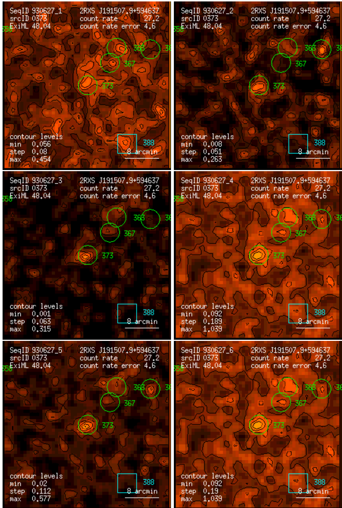
Figure 373: RASS 930627: detection 0373: band rate images, Gaussian filter: (1) PSPC channels 11 – 41, (2) 52 – 90, (3) 91 – 201, (4) 11 – 235, (5) 52 – 201, (6) 11 – 201. Broad band rates in counts/ks. Band rate contour levels in counts/ks/arcmin 2 .
