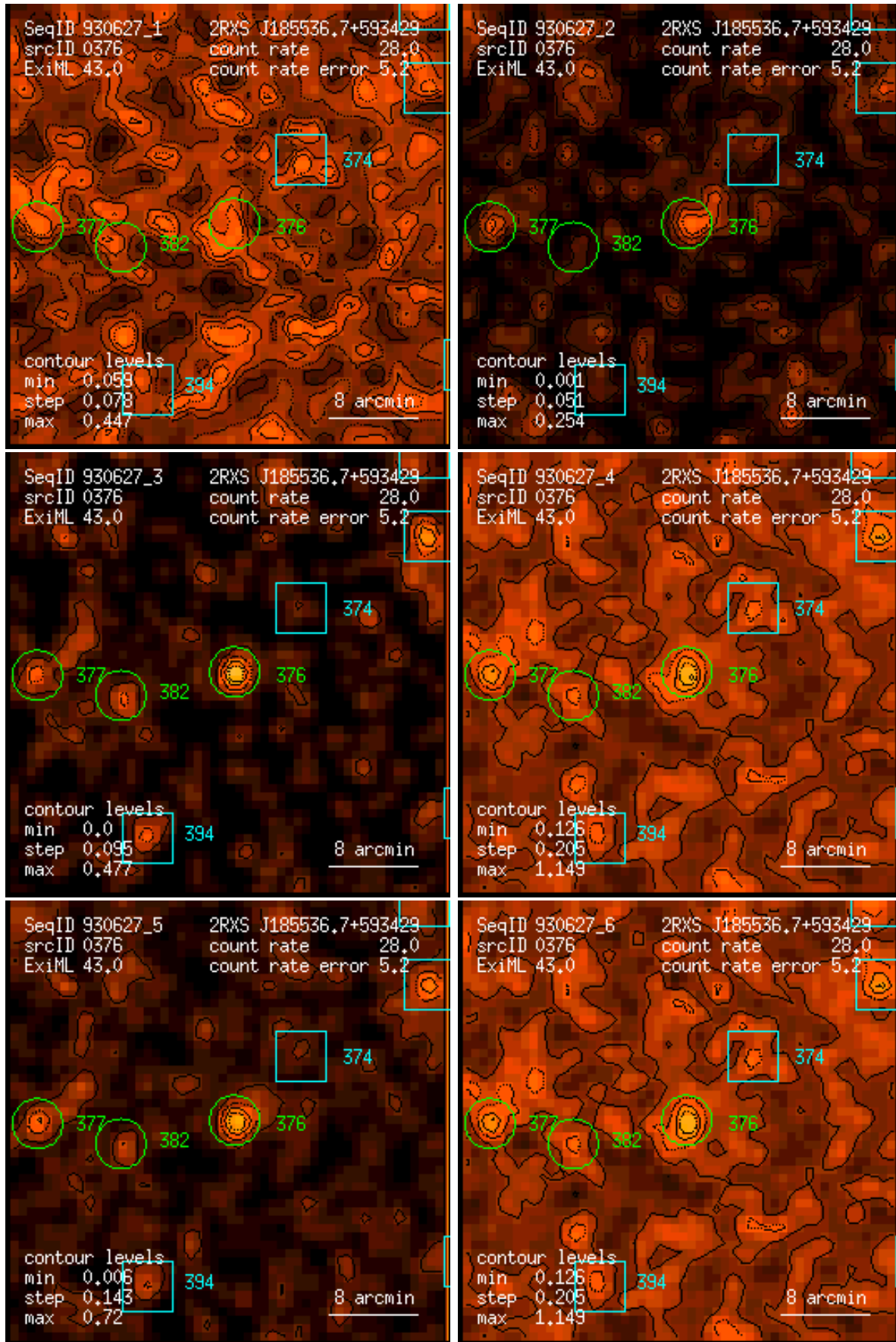
Figure 376: RASS 930627: detection 0376: band rate images, Gaussian filter: (1) PSPC channels 11 – 41, (2) 52 – 90, (3) 91 – 201, (4) 11 – 235, (5) 52 – 201, (6) 11 – 201. Broad band rates in counts/ks. Band rate contour levels in counts/ks/arcmin 2 .
