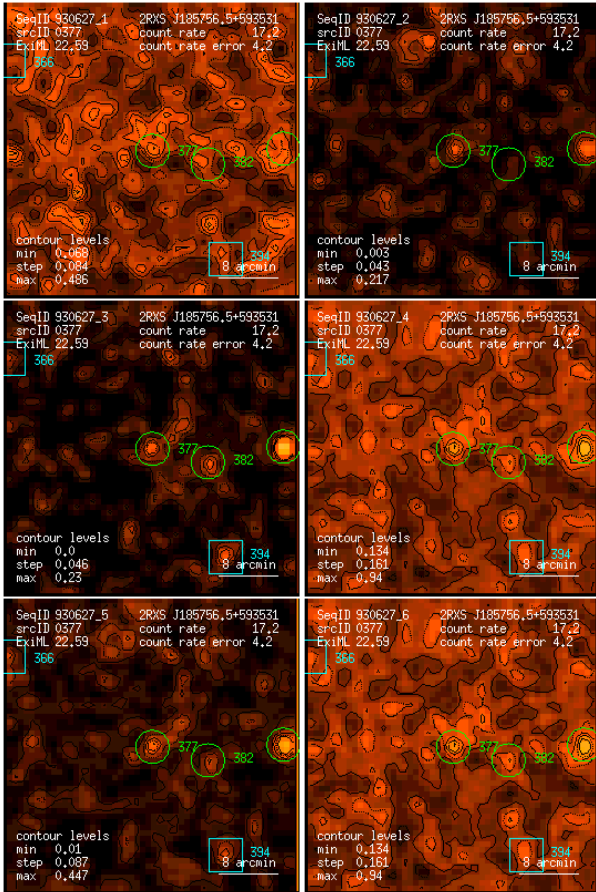
Figure 377: RASS 930627: detection 0377: band rate images, Gaussian filter: (1) PSPC channels 11 – 41, (2) 52 – 90, (3) 91 – 201, (4) 11 – 235, (5) 52 – 201, (6) 11 – 201. Broad band rates in counts/ks. Band rate contour levels in counts/ks/arcmin 2 .
