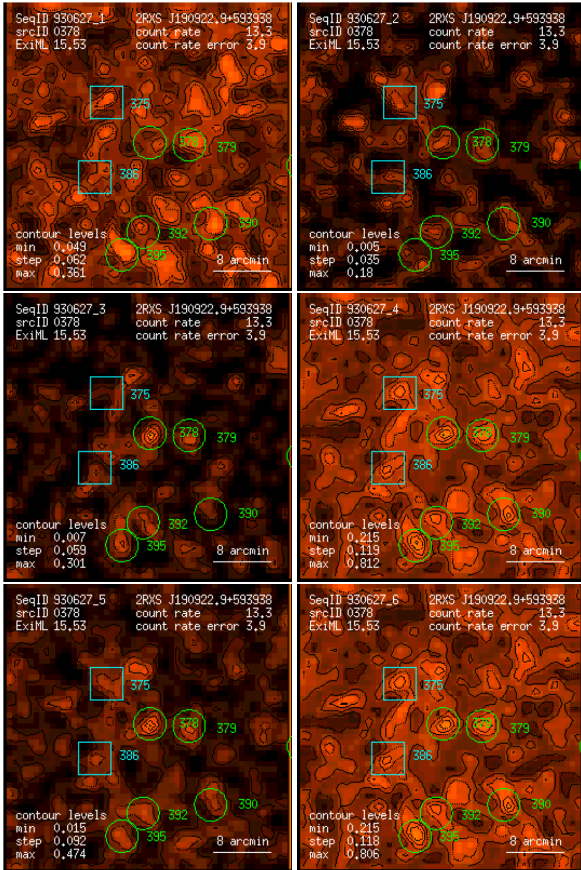
Figure 378: RASS 930627: detection 0378: band rate images, Gaussian filter: (1) PSPC channels 11 – 41, (2) 52 – 90, (3) 91 – 201, (4) 11 – 235, (5) 52 – 201, (6) 11 – 201. Broad band rates in counts/ks. Band rate contour levels in counts/ks/arcmin 2 .
