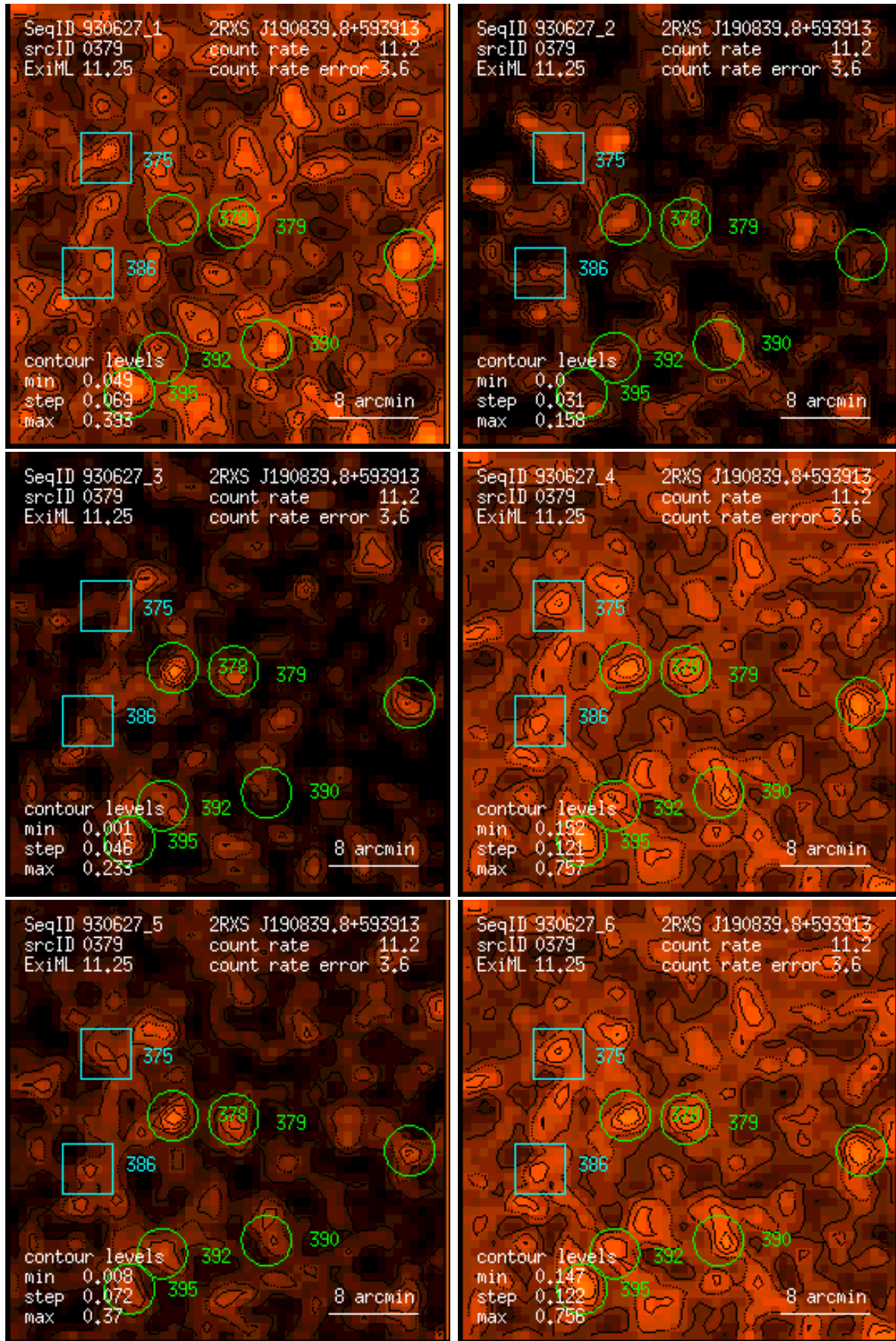
Figure 379: RASS 930627: detection 0379: band rate images, Gaussian filter: (1) PSPC channels 11 – 41, (2) 52 – 90, (3) 91 – 201, (4) 11 – 235, (5) 52 – 201, (6) 11 – 201. Broad band rates in counts/ks. Band rate contour levels in counts/ks/arcmin 2 .
