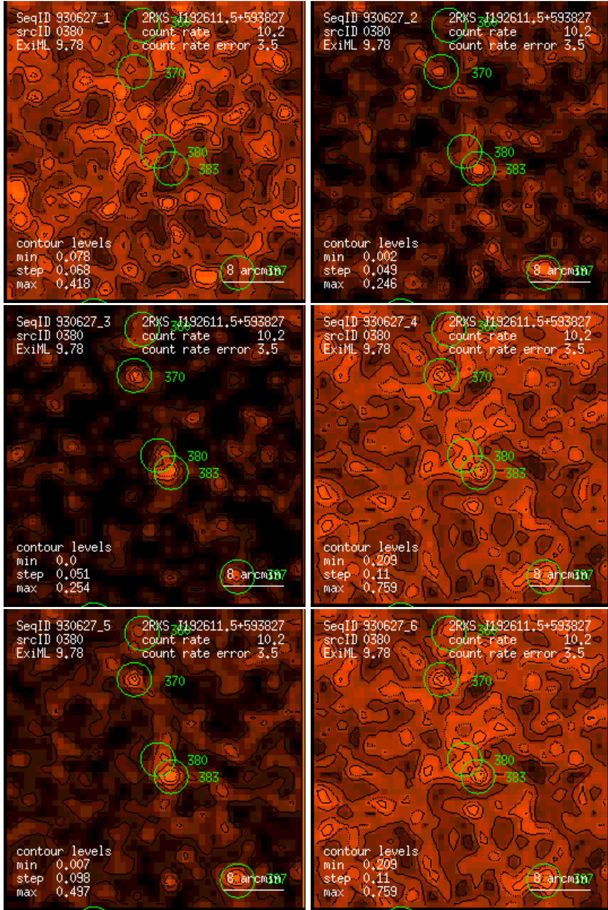
Figure 380: RASS 930627: detection 0380: band rate images, Gaussian filter: (1) PSPC channels 11 – 41, (2) 52 – 90, (3) 91 – 201, (4) 11 – 235, (5) 52 – 201, (6) 11 – 201. Broad band rates in counts/ks. Band rate contour levels in counts/ks/arcmin 2 .
