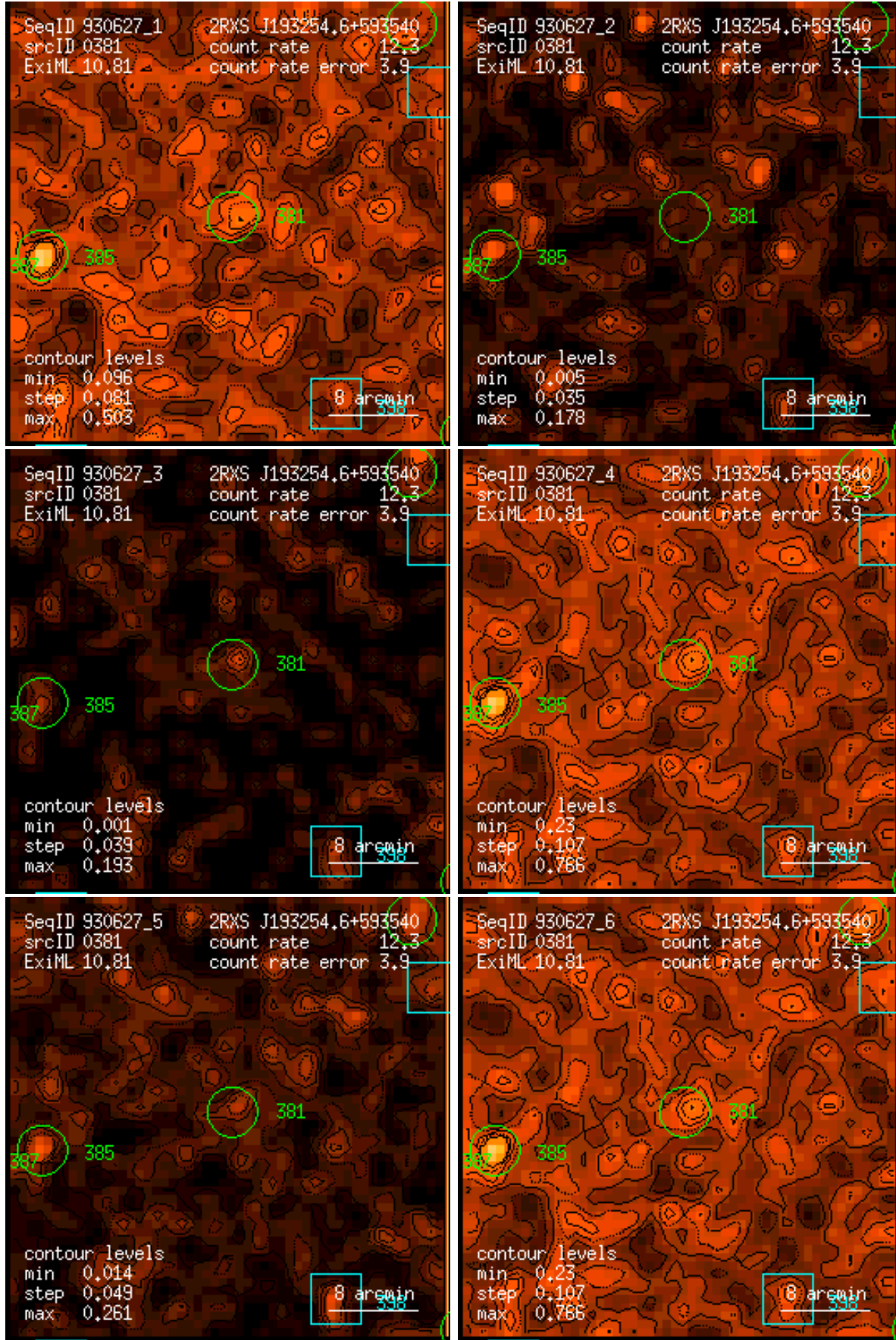
Figure 381: RASS 930627: detection 0381: band rate images, Gaussian filter: (1) PSPC channels 11 – 41, (2) 52 – 90, (3) 91 – 201, (4) 11 – 235, (5) 52 – 201, (6) 11 – 201. Broad band rates in counts/ks. Band rate contour levels in counts/ks/arcmin 2 .
