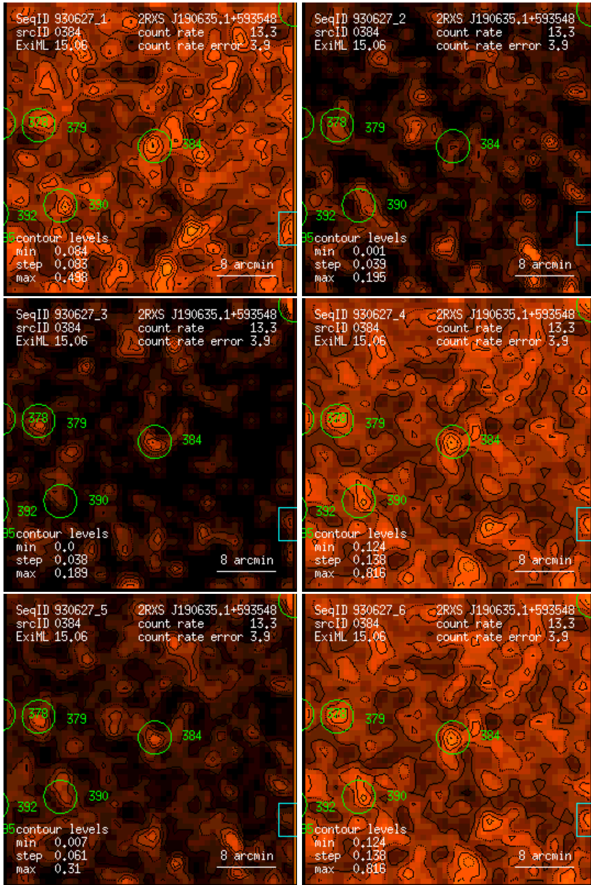
Figure 384: RASS 930627: detection 0384: band rate images, Gaussian filter: (1) PSPC channels 11 – 41, (2) 52 – 90, (3) 91 – 201, (4) 11 – 235, (5) 52 – 201, (6) 11 – 201. Broad band rates in counts/ks. Band rate contour levels in counts/ks/arcmin 2 .
