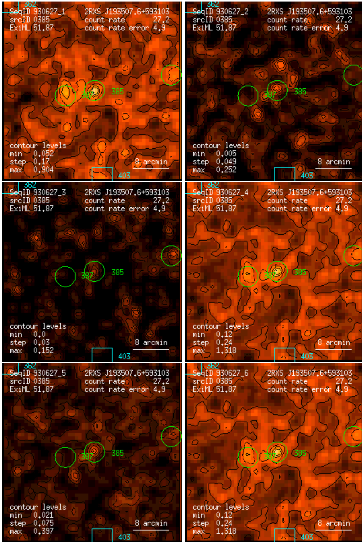
Figure 385: RASS 930627: detection 0385: band rate images, Gaussian filter: (1) PSPC channels 11 – 41, (2) 52 – 90, (3) 91 – 201, (4) 11 – 235, (5) 52 – 201, (6) 11 – 201. Broad band rates in counts/ks. Band rate contour levels in counts/ks/arcmin 2 .
