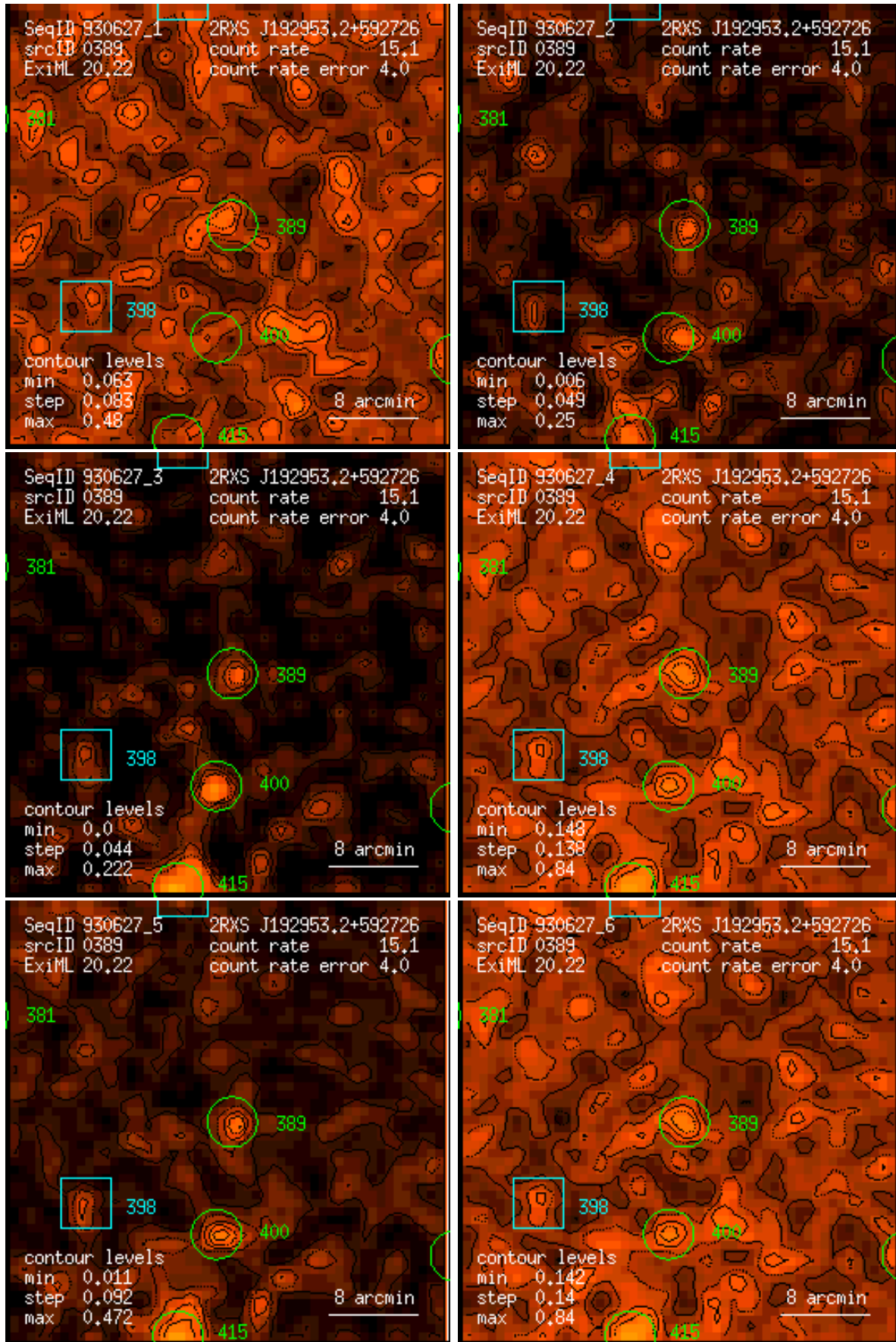
Figure 389: RASS 930627: detection 0389: band rate images, Gaussian filter: (1) PSPC channels 11 – 41, (2) 52 – 90, (3) 91 – 201, (4) 11 – 235, (5) 52 – 201, (6) 11 – 201. Broad band rates in counts/ks. Band rate contour levels in counts/ks/arcmin 2 .
