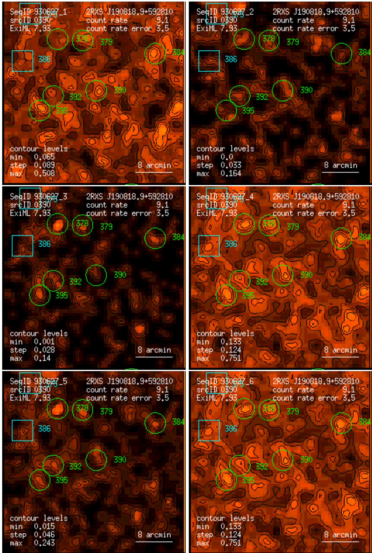
Figure 390: RASS 930627: detection 0390: band rate images, Gaussian filter: (1) PSPC channels 11 – 41, (2) 52 – 90, (3) 91 – 201, (4) 11 – 235, (5) 52 – 201, (6) 11 – 201. Broad band rates in counts/ks. Band rate contour levels in counts/ks/arcmin 2 .
