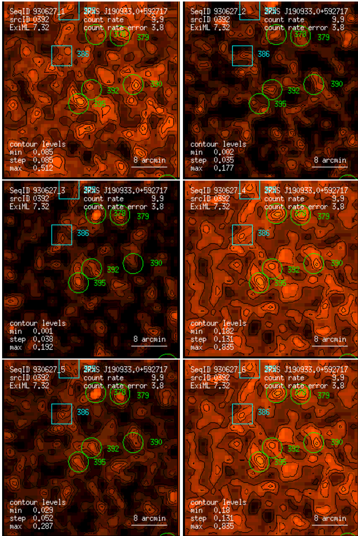
Figure 392: RASS 930627: detection 0392: band rate images, Gaussian filter: (1) PSPC channels 11 – 41, (2) 52 – 90, (3) 91 – 201, (4) 11 – 235, (5) 52 – 201, (6) 11 – 201. Broad band rates in counts/ks. Band rate contour levels in counts/ks/arcmin 2 .
