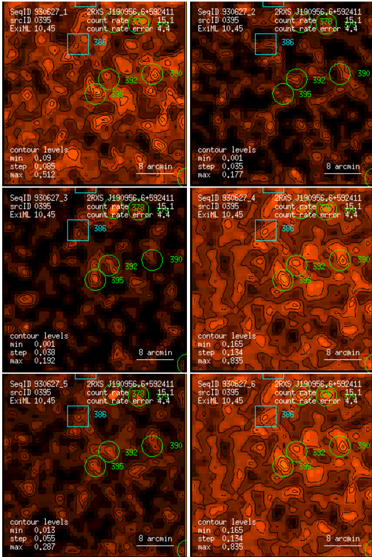
Figure 395: RASS 930627: detection 0395: band rate images, Gaussian filter: (1) PSPC channels 11 – 41, (2) 52 – 90, (3) 91 – 201, (4) 11 – 235, (5) 52 – 201, (6) 11 – 201. Broad band rates in counts/ks. Band rate contour levels in counts/ks/arcmin 2 .
