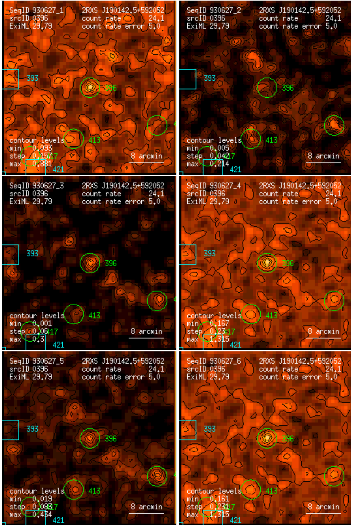
Figure 396: RASS 930627: detection 0396: band rate images, Gaussian filter: (1) PSPC channels 11 – 41, (2) 52 – 90, (3) 91 – 201, (4) 11 – 235, (5) 52 – 201, (6) 11 – 201. Broad band rates in counts/ks. Band rate contour levels in counts/ks/arcmin 2 .
