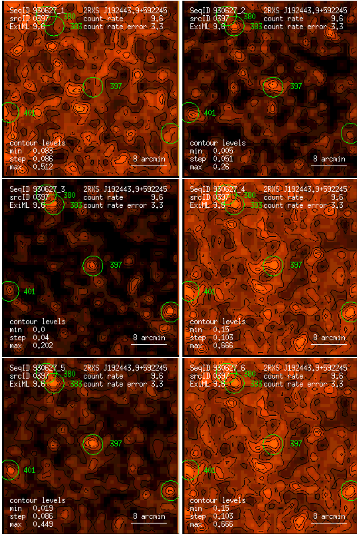
Figure 397: RASS 930627: detection 0397: band rate images, Gaussian filter: (1) PSPC channels 11 – 41, (2) 52 – 90, (3) 91 – 201, (4) 11 – 235, (5) 52 – 201, (6) 11 – 201. Broad band rates in counts/ks. Band rate contour levels in counts/ks/arcmin 2 .
