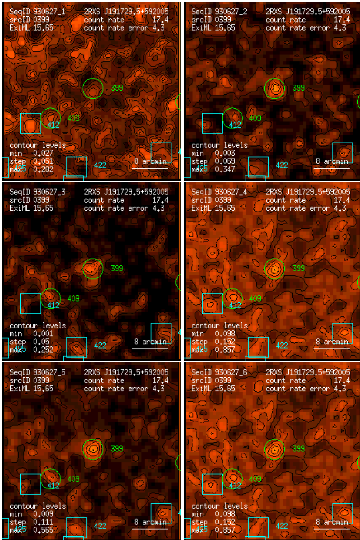
Figure 399: RASS 930627: detection 0399: band rate images, Gaussian filter: (1) PSPC channels 11 – 41, (2) 52 – 90, (3) 91 – 201, (4) 11 – 235, (5) 52 – 201, (6) 11 – 201. Broad band rates in counts/ks. Band rate contour levels in counts/ks/arcmin 2 .
