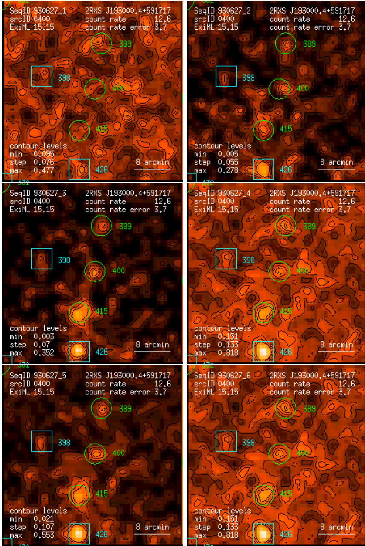
Figure 400: RASS 930627: detection 0400: band rate images, Gaussian filter: (1) PSPC channels 11 – 41, (2) 52 – 90, (3) 91 – 201, (4) 11 – 235, (5) 52 – 201, (6) 11 – 201. Broad band rates in counts/ks. Band rate contour levels in counts/ks/arcmin 2 .
