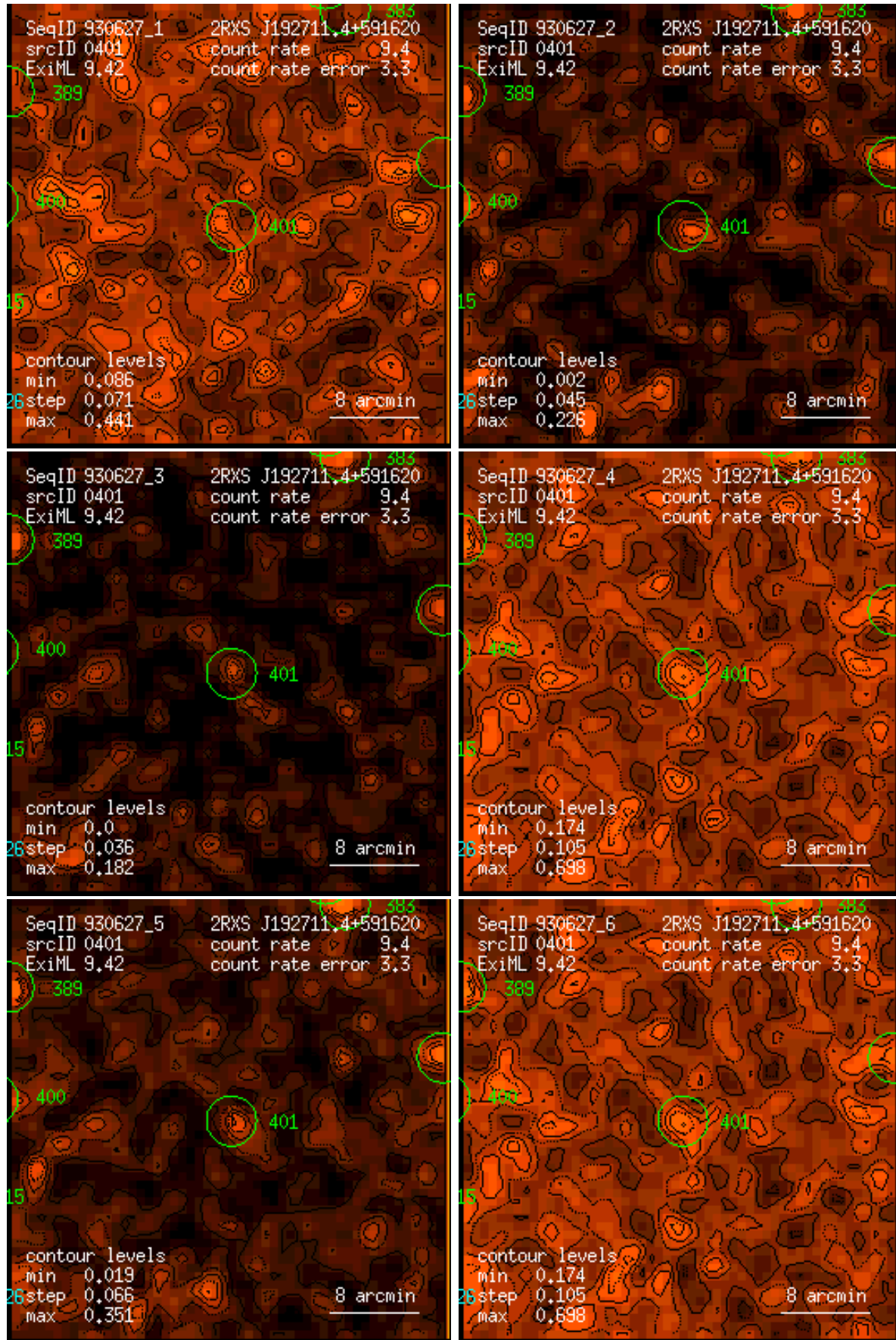
Figure 401: RASS 930627: detection 0401: band rate images, Gaussian filter: (1) PSPC channels 11 – 41, (2) 52 – 90, (3) 91 – 201, (4) 11 – 235, (5) 52 – 201, (6) 11 – 201. Broad band rates in counts/ks. Band rate contour levels in counts/ks/arcmin 2 .
