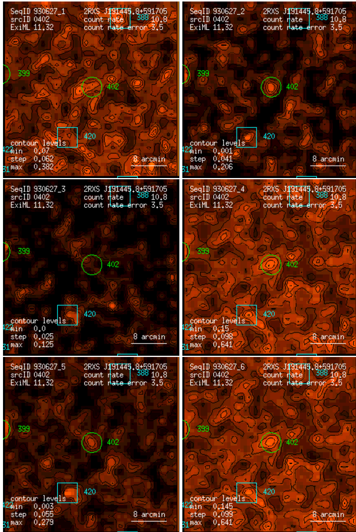
Figure 402: RASS 930627: detection 0402: band rate images, Gaussian filter: (1) PSPC channels 11 – 41, (2) 52 – 90, (3) 91 – 201, (4) 11 – 235, (5) 52 – 201, (6) 11 – 201. Broad band rates in counts/ks. Band rate contour levels in counts/ks/arcmin 2 .
