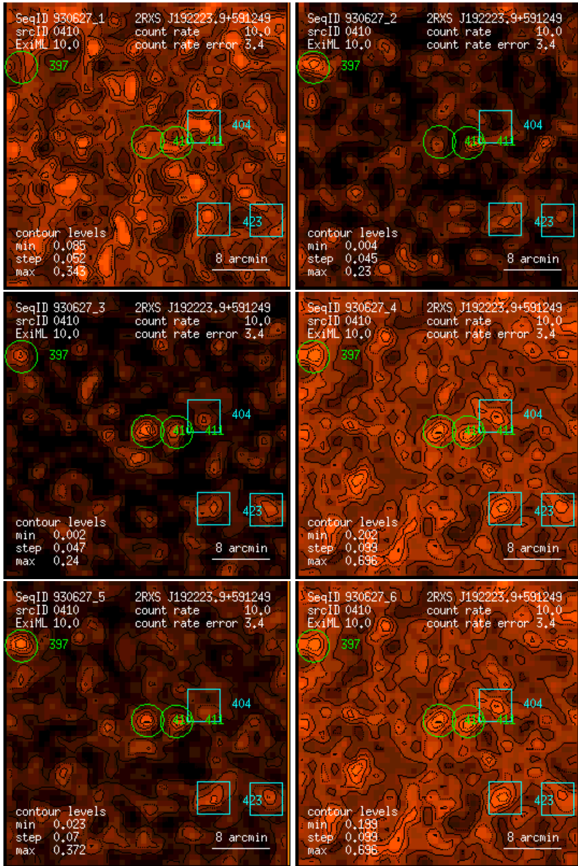
Figure 410: RASS 930627: detection 0410: band rate images, Gaussian filter: (1) PSPC channels 11 – 41, (2) 52 – 90, (3) 91 – 201, (4) 11 – 235, (5) 52 – 201, (6) 11 – 201. Broad band rates in counts/ks. Band rate contour levels in counts/ks/arcmin 2 .
