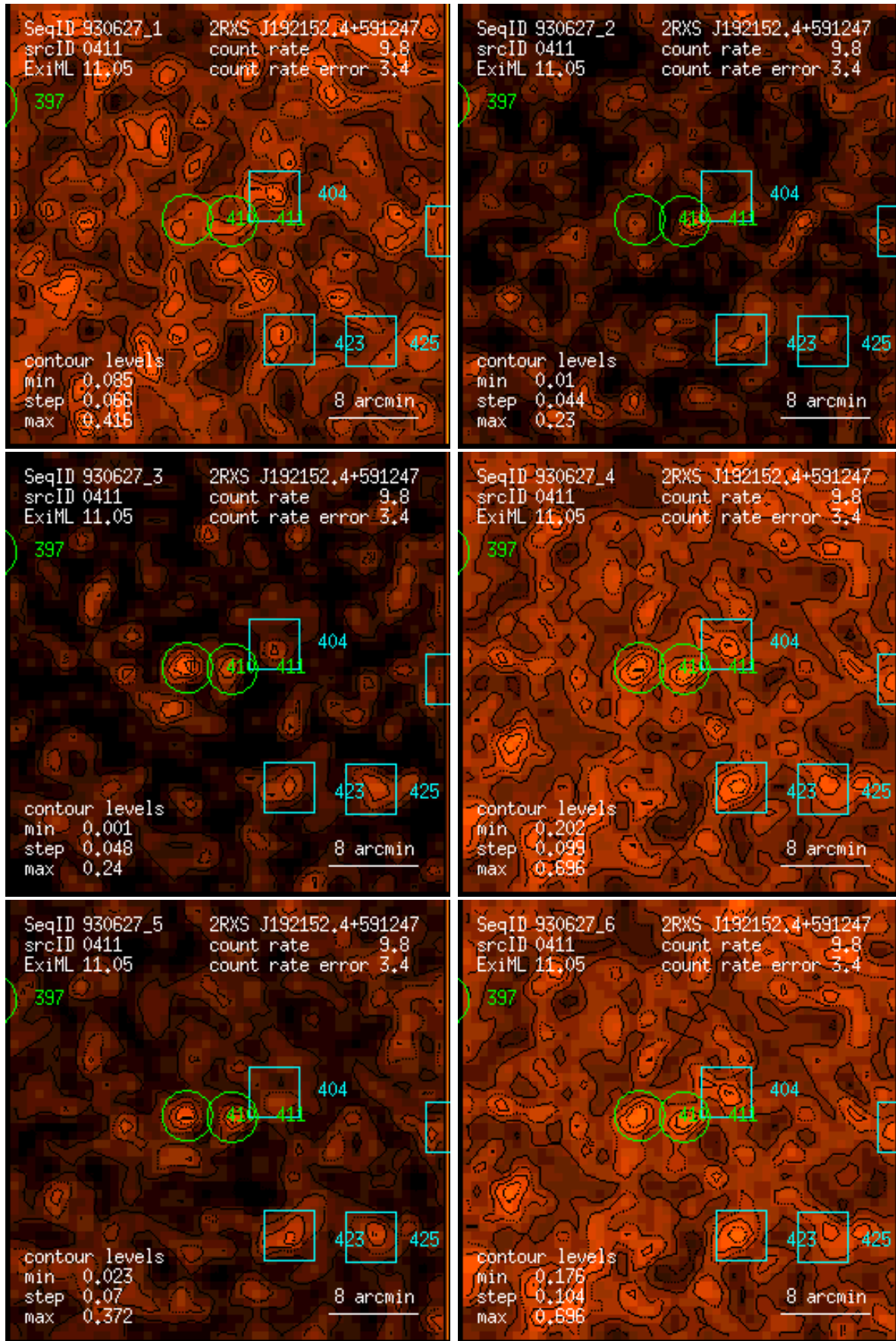
Figure 411: RASS 930627: detection 0411: band rate images, Gaussian filter: (1) PSPC channels 11 – 41, (2) 52 – 90, (3) 91 – 201, (4) 11 – 235, (5) 52 – 201, (6) 11 – 201. Broad band rates in counts/ks. Band rate contour levels in counts/ks/arcmin 2 .
