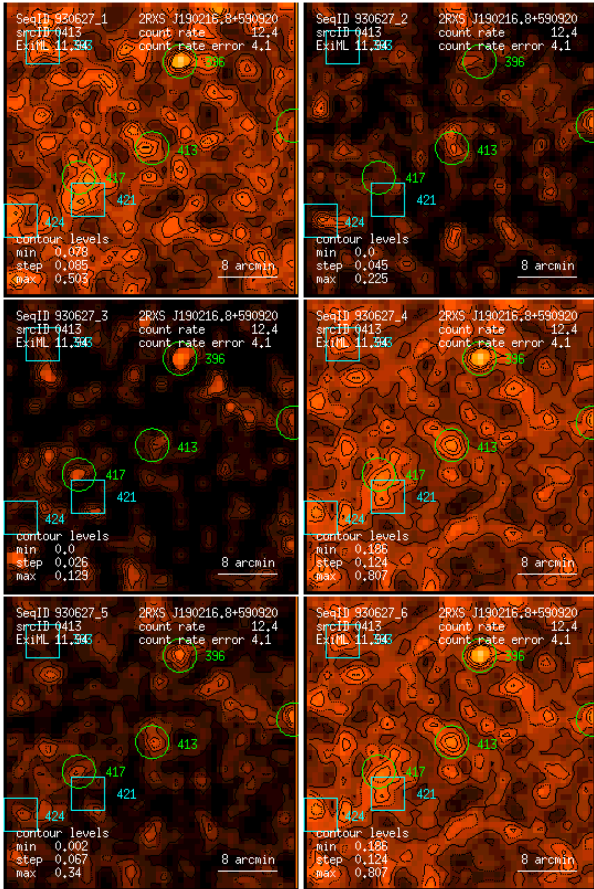
Figure 413: RASS 930627: detection 0413: band rate images, Gaussian filter: (1) PSPC channels 11 – 41, (2) 52 – 90, (3) 91 – 201, (4) 11 – 235, (5) 52 – 201, (6) 11 – 201. Broad band rates in counts/ks. Band rate contour levels in counts/ks/arcmin 2 .
