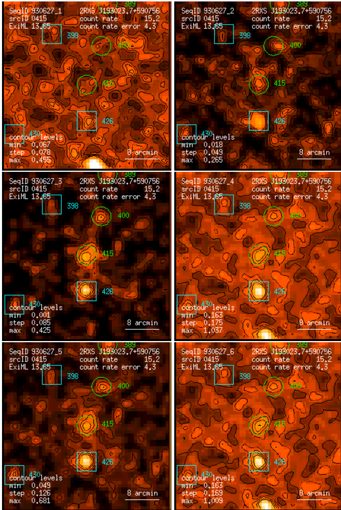
Figure 415: RASS 930627: detection 0415: band rate images, Gaussian filter: (1) PSPC channels 11 – 41, (2) 52 – 90, (3) 91 – 201, (4) 11 – 235, (5) 52 – 201, (6) 11 – 201. Broad band rates in counts/ks. Band rate contour levels in counts/ks/arcmin 2 .
