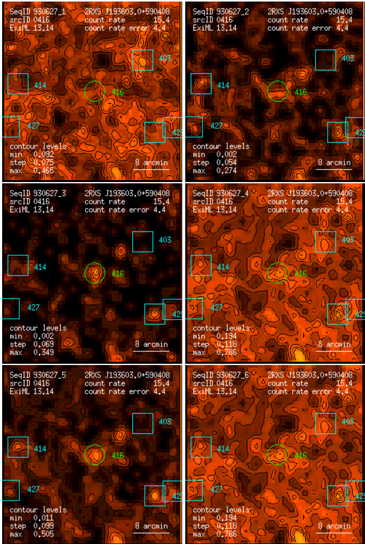
Figure 416: RASS 930627: detection 0416: band rate images, Gaussian filter: (1) PSPC channels 11 – 41, (2) 52 – 90, (3) 91 – 201, (4) 11 – 235, (5) 52 – 201, (6) 11 – 201. Broad band rates in counts/ks. Band rate contour levels in counts/ks/arcmin 2 .
