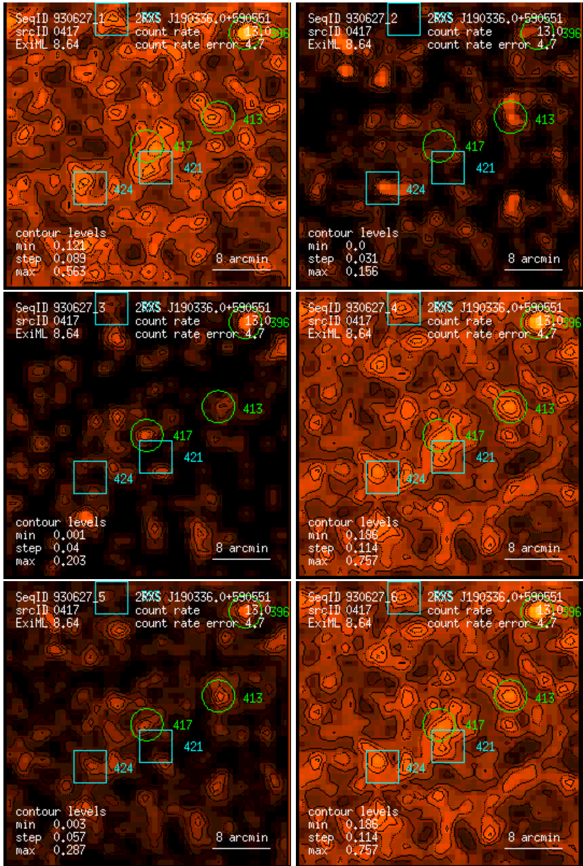
Figure 417: RASS 930627: detection 0417: band rate images, Gaussian filter: (1) PSPC channels 11 – 41, (2) 52 – 90, (3) 91 – 201, (4) 11 – 235, (5) 52 – 201, (6) 11 – 201. Broad band rates in counts/ks. Band rate contour levels in counts/ks/arcmin 2 .
