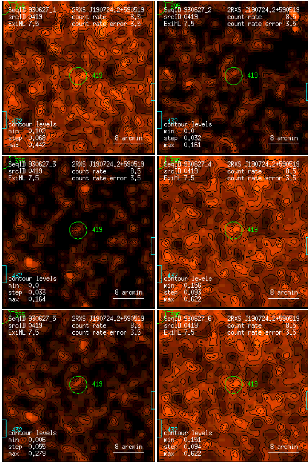
Figure 419: RASS 930627: detection 0419: band rate images, Gaussian filter: (1) PSPC channels 11 – 41, (2) 52 – 90, (3) 91 – 201, (4) 11 – 235, (5) 52 – 201, (6) 11 – 201. Broad band rates in counts/ks. Band rate contour levels in counts/ks/arcmin 2 .
