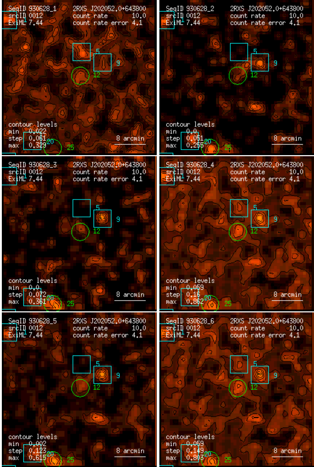
Figure 12: RASS 930628: detection 0012: band rate images, Gaussian filter: (1) PSPC channels 11 – 41, (2) 52 – 90, (3) 91 – 201, (4) 11 – 235, (5) 52 – 201, (6) 11 – 201. Broad band rates in counts/ks. Band rate contour levels in counts/ks/arcmin 2 .
