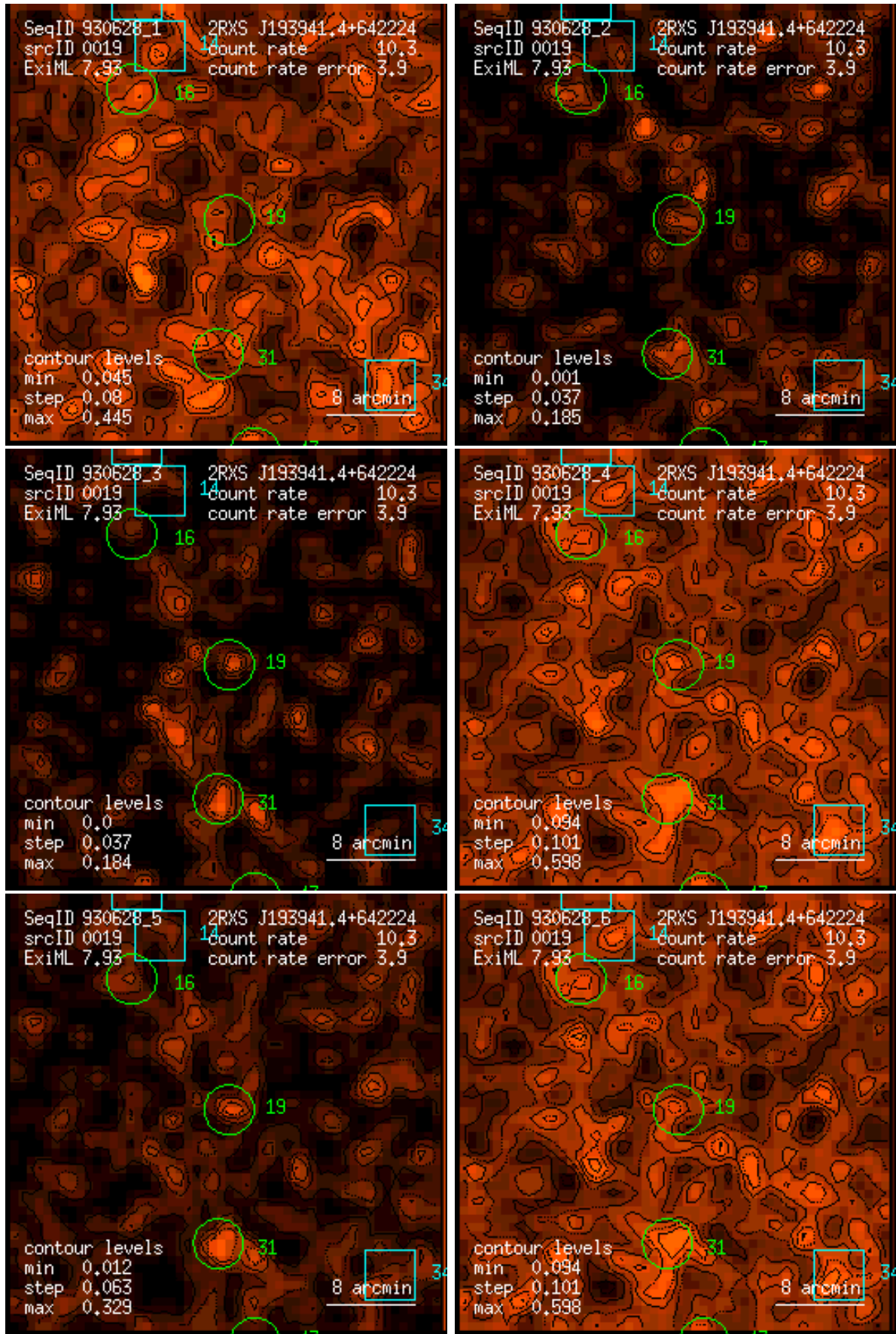
Figure 19: RASS 930628: detection 0019: band rate images, Gaussian filter: (1) PSPC channels 11 – 41, (2) 52 – 90, (3) 91 – 201, (4) 11 – 235, (5) 52 – 201, (6) 11 – 201. Broad band rates in counts/ks. Band rate contour levels in counts/ks/arcmin 2 .
