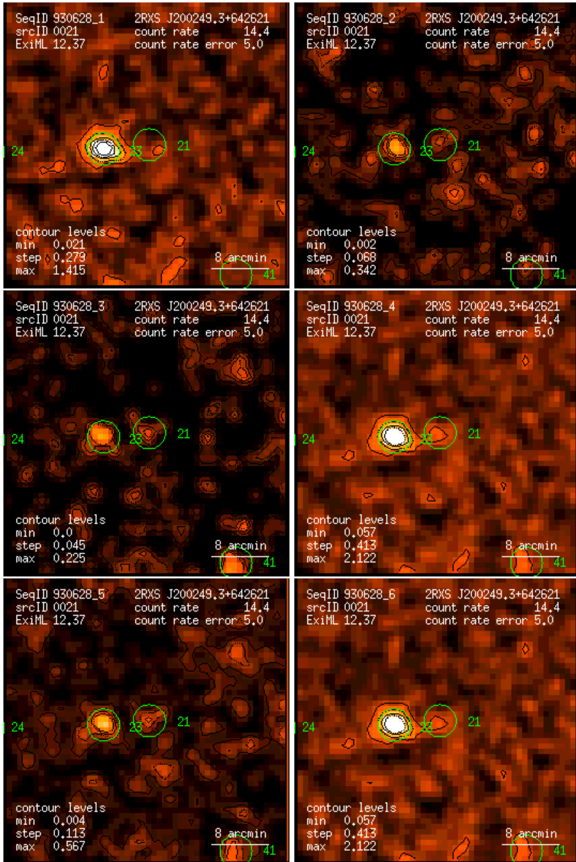
Figure 21: RASS 930628: detection 0021: band rate images, Gaussian filter: (1) PSPC channels 11 – 41, (2) 52 – 90, (3) 91 – 201, (4) 11 – 235, (5) 52 – 201, (6) 11 – 201. Broad band rates in counts/ks. Band rate contour levels in counts/ks/arcmin 2 .
