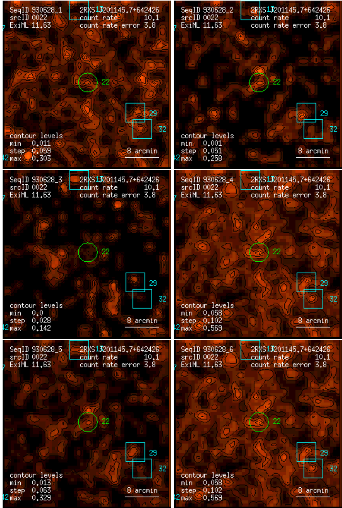
Figure 22: RASS 930628: detection 0022: band rate images, Gaussian filter: (1) PSPC channels 11 – 41, (2) 52 – 90, (3) 91 – 201, (4) 11 – 235, (5) 52 – 201, (6) 11 – 201. Broad band rates in counts/ks. Band rate contour levels in counts/ks/arcmin 2 .
