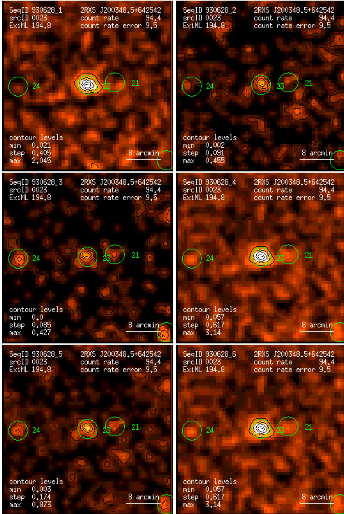
Figure 23: RASS 930628: detection 0023: band rate images, Gaussian filter: (1) PSPC channels 11 – 41, (2) 52 – 90, (3) 91 – 201, (4) 11 – 235, (5) 52 – 201, (6) 11 – 201. Broad band rates in counts/ks. Band rate contour levels in counts/ks/arcmin 2 .
