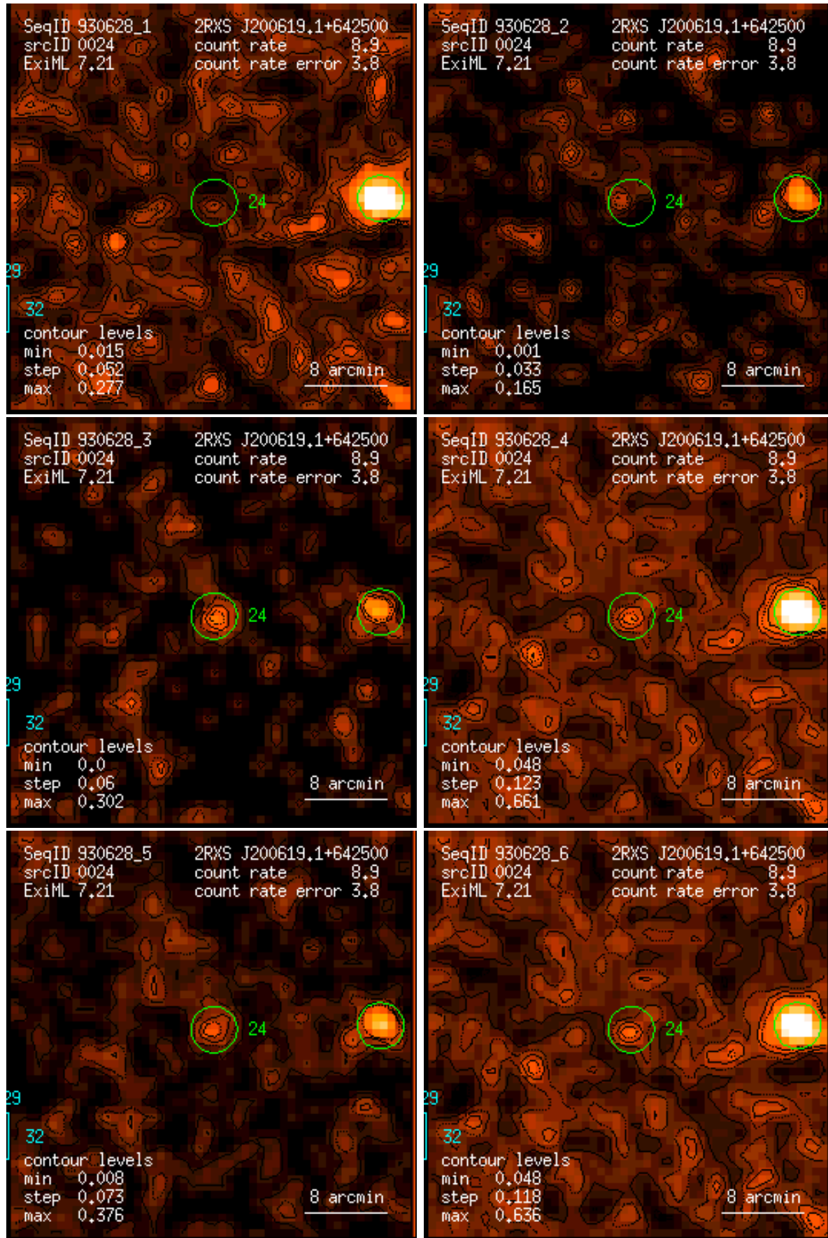
Figure 24: RASS 930628: detection 0024: band rate images, Gaussian filter: (1) PSPC channels 11 – 41, (2) 52 – 90, (3) 91 – 201, (4) 11 – 235, (5) 52 – 201, (6) 11 – 201. Broad band rates in counts/ks. Band rate contour levels in counts/ks/arcmin 2 .
