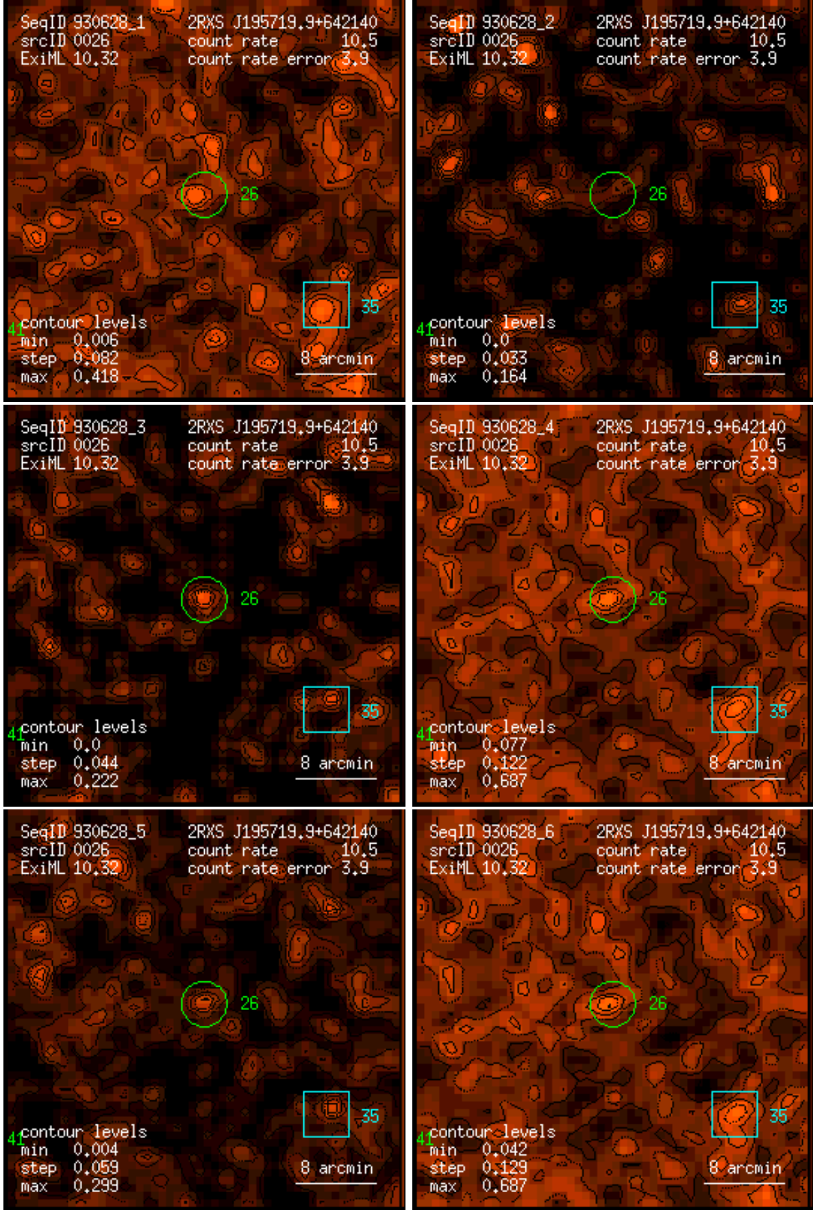
Figure 26: RASS 930628: detection 0026: band rate images, Gaussian filter: (1) PSPC channels 11 – 41, (2) 52 – 90, (3) 91 – 201, (4) 11 – 235, (5) 52 – 201, (6) 11 – 201. Broad band rates in counts/ks. Band rate contour levels in counts/ks/arcmin 2 .
