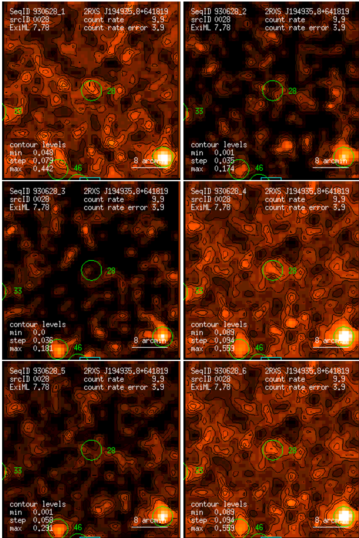
Figure 28: RASS 930628: detection 0028: band rate images, Gaussian filter: (1) PSPC channels 11 – 41, (2) 52 – 90, (3) 91 – 201, (4) 11 – 235, (5) 52 – 201, (6) 11 – 201. Broad band rates in counts/ks. Band rate contour levels in counts/ks/arcmin 2 .
