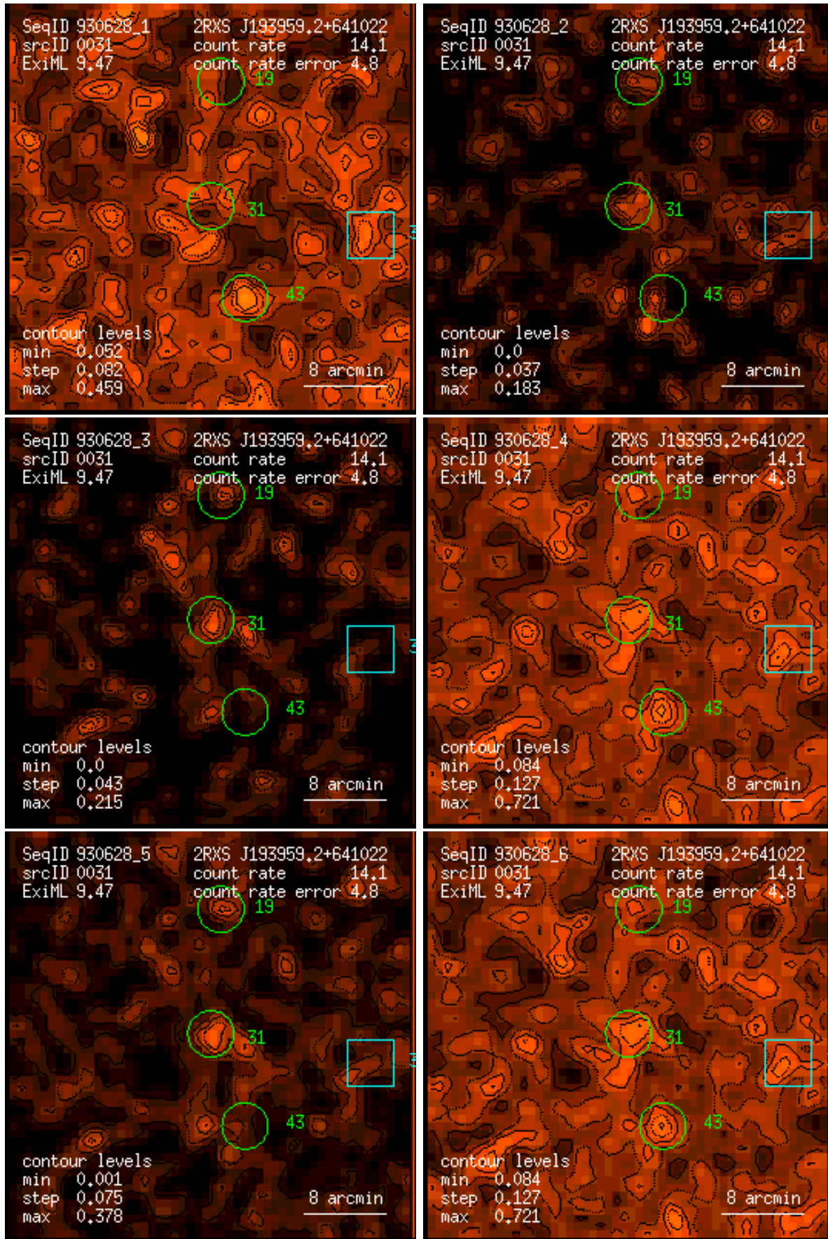
Figure 31: RASS 930628: detection 0031: band rate images, Gaussian filter: (1) PSPC channels 11 – 41, (2) 52 – 90, (3) 91 – 201, (4) 11 – 235, (5) 52 – 201, (6) 11 – 201. Broad band rates in counts/ks. Band rate contour levels in counts/ks/arcmin 2 .
