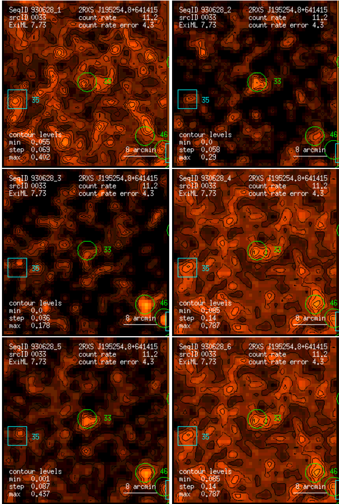
Figure 33: RASS 930628: detection 0033: band rate images, Gaussian filter: (1) PSPC channels 11 – 41, (2) 52 – 90, (3) 91 – 201, (4) 11 – 235, (5) 52 – 201, (6) 11 – 201. Broad band rates in counts/ks. Band rate contour levels in counts/ks/arcmin 2 .
