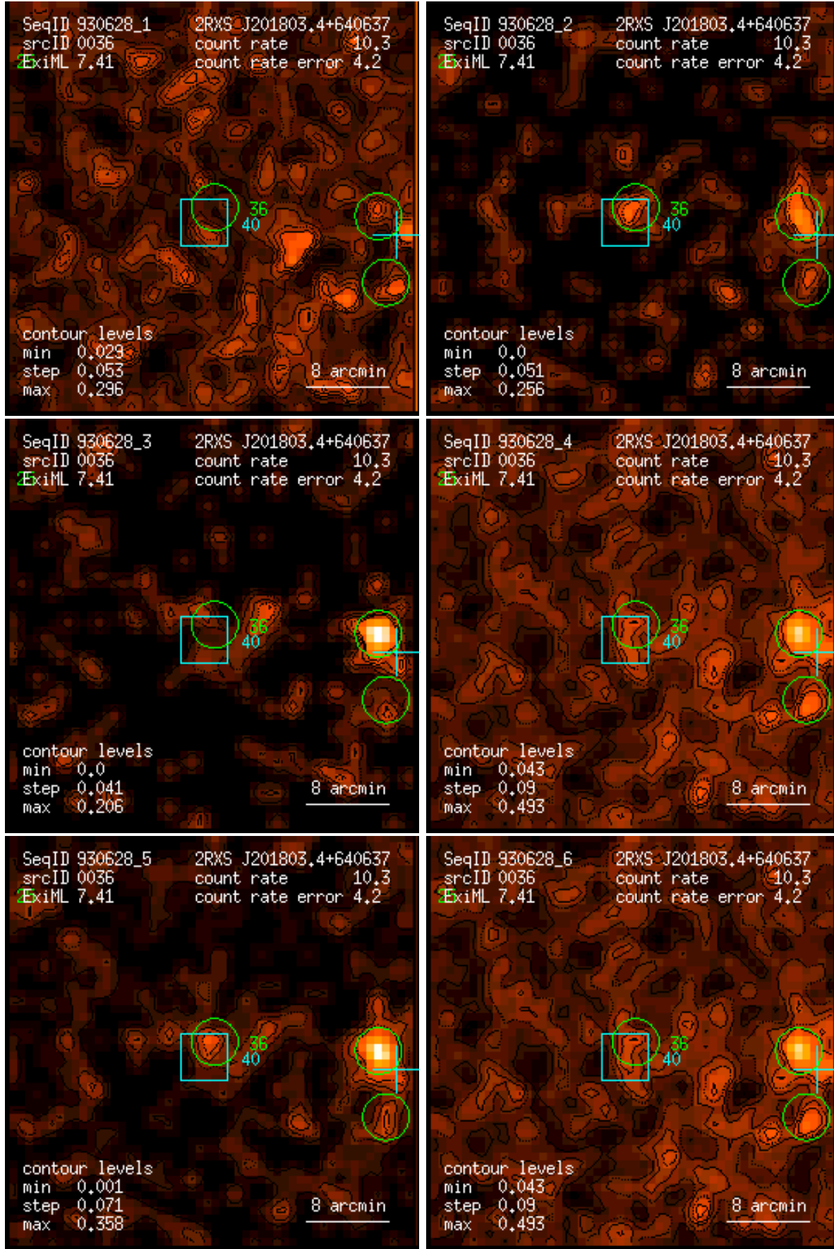
Figure 36: RASS 930628: detection 0036: band rate images, Gaussian filter: (1) PSPC channels 11 – 41, (2) 52 – 90, (3) 91 – 201, (4) 11 – 235, (5) 52 – 201, (6) 11 – 201. Broad band rates in counts/ks. Band rate contour levels in counts/ks/arcmin 2 .
