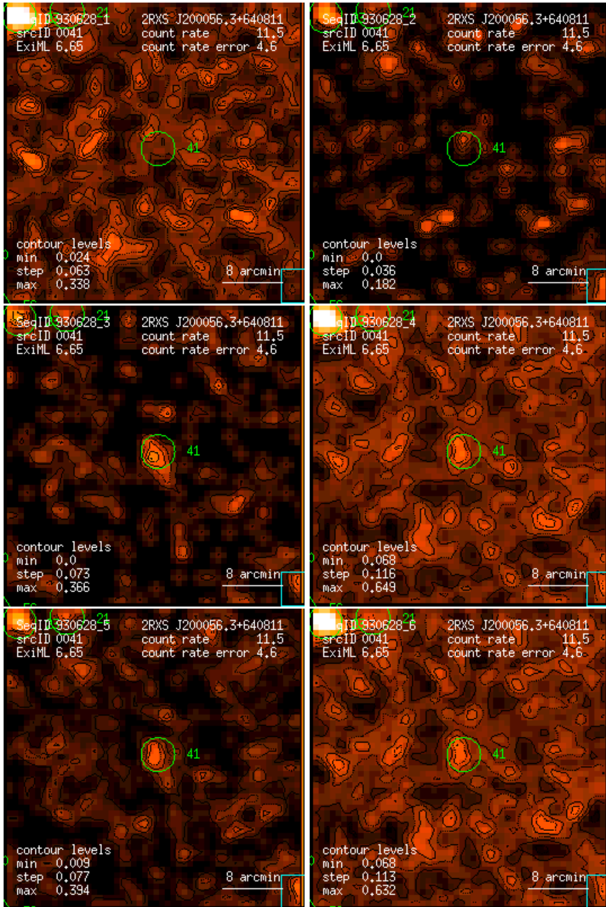
Figure 41: RASS 930628: detection 0041: band rate images, Gaussian filter: (1) PSPC channels 11 – 41, (2) 52 – 90, (3) 91 – 201, (4) 11 – 235, (5) 52 – 201, (6) 11 – 201. Broad band rates in counts/ks. Band rate contour levels in counts/ks/arcmin 2 .
