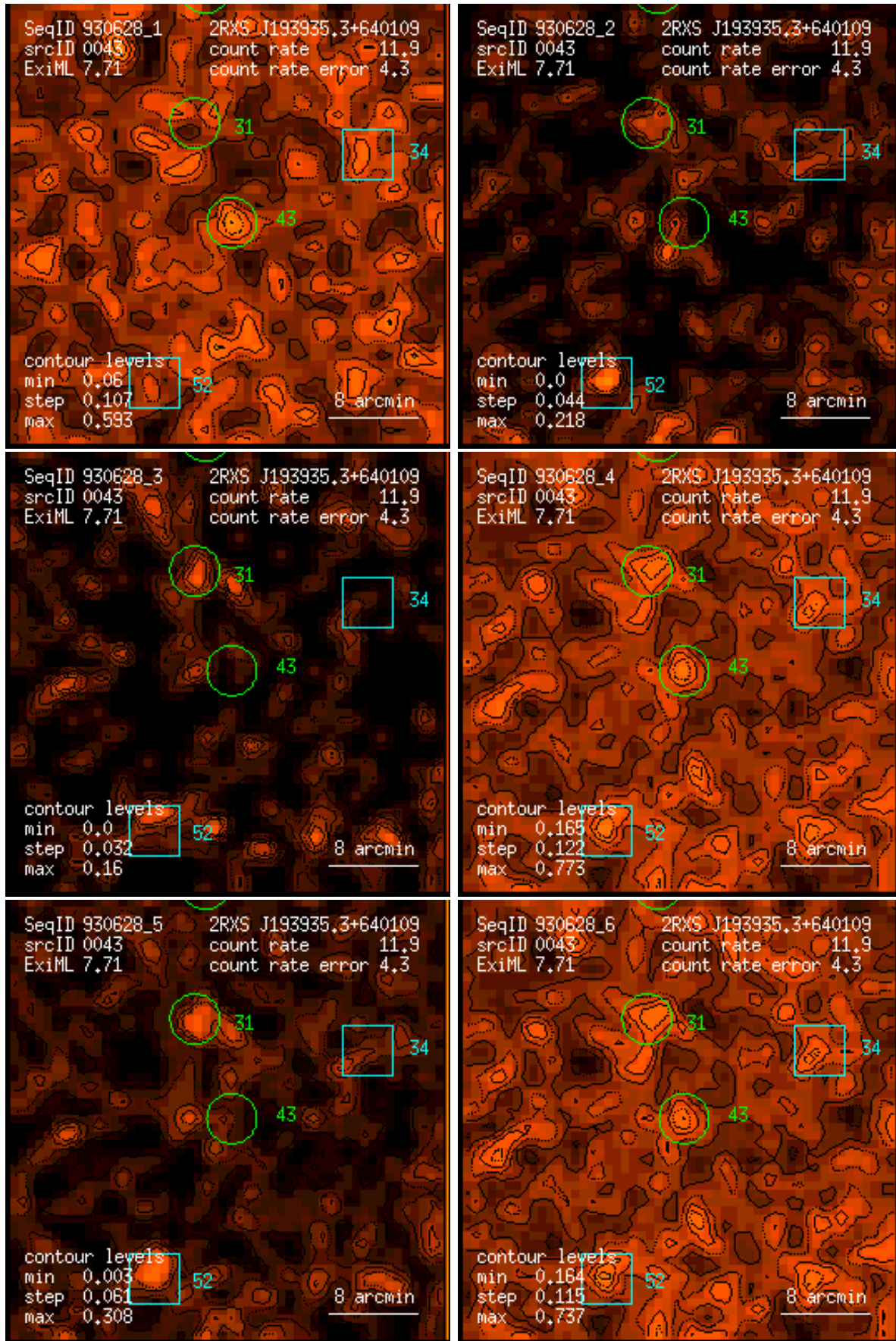
Figure 43: RASS 930628: detection 0043: band rate images, Gaussian filter: (1) PSPC channels 11 – 41, (2) 52 – 90, (3) 91 – 201, (4) 11 – 235, (5) 52 – 201, (6) 11 – 201. Broad band rates in counts/ks. Band rate contour levels in counts/ks/arcmin 2 .
