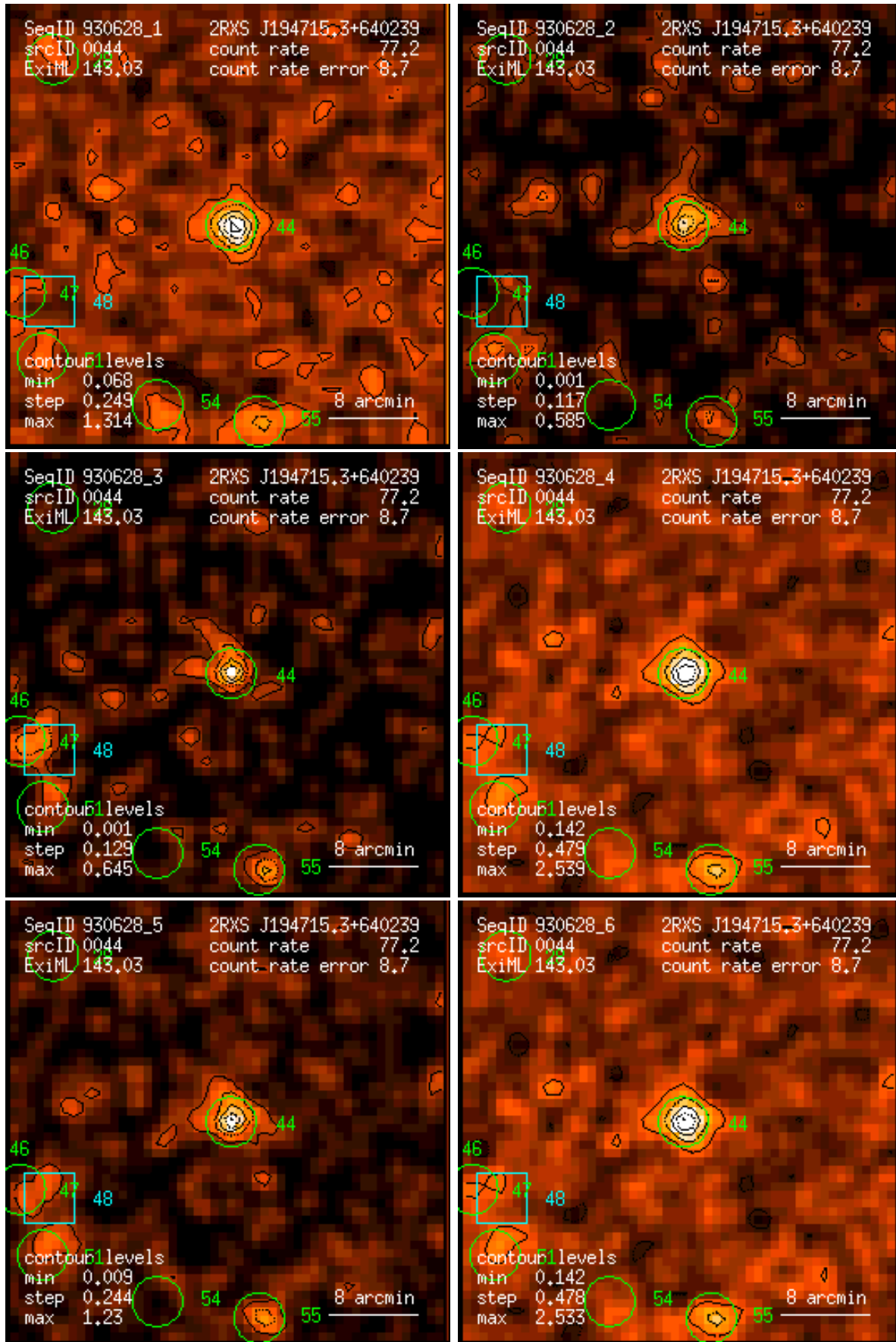
Figure 44: RASS 930628: detection 0044: band rate images, Gaussian filter: (1) PSPC channels 11 – 41, (2) 52 – 90, (3) 91 – 201, (4) 11 – 235, (5) 52 – 201, (6) 11 – 201. Broad band rates in counts/ks. Band rate contour levels in counts/ks/arcmin 2 .
