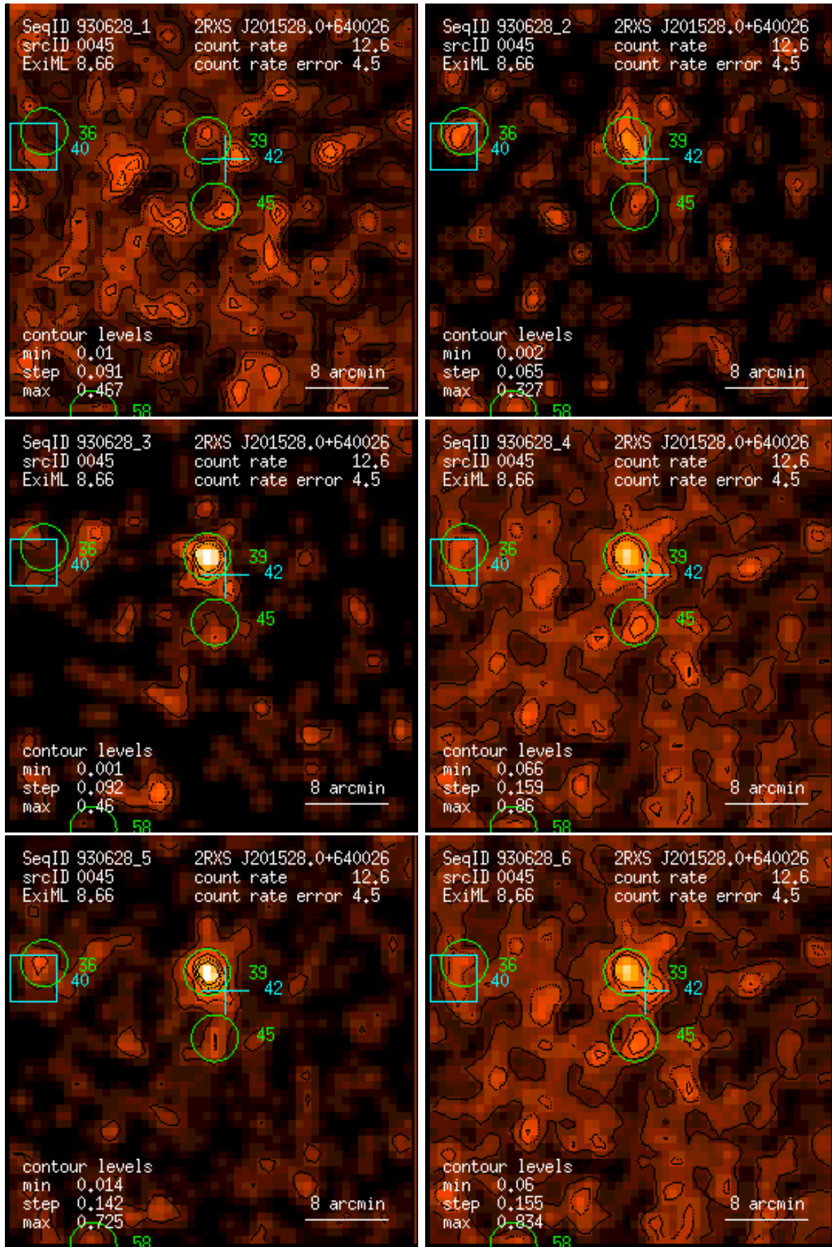
Figure 45: RASS 930628: detection 0045: band rate images, Gaussian filter: (1) PSPC channels 11 – 41, (2) 52 – 90, (3) 91 – 201, (4) 11 – 235, (5) 52 – 201, (6) 11 – 201. Broad band rates in counts/ks. Band rate contour levels in counts/ks/arcmin 2 .
