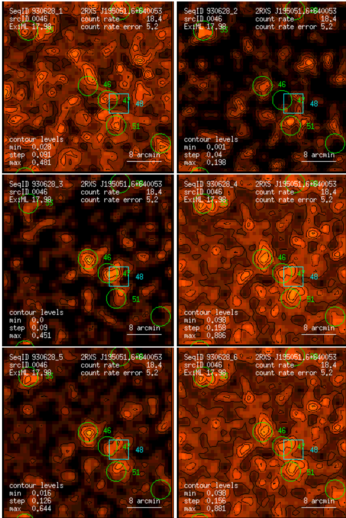
Figure 46: RASS 930628: detection 0046: band rate images, Gaussian filter: (1) PSPC channels 11 – 41, (2) 52 – 90, (3) 91 – 201, (4) 11 – 235, (5) 52 – 201, (6) 11 – 201. Broad band rates in counts/ks. Band rate contour levels in counts/ks/arcmin 2 .
